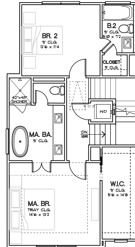
THIRD FLOOR PLAN PLAN 1850 L
