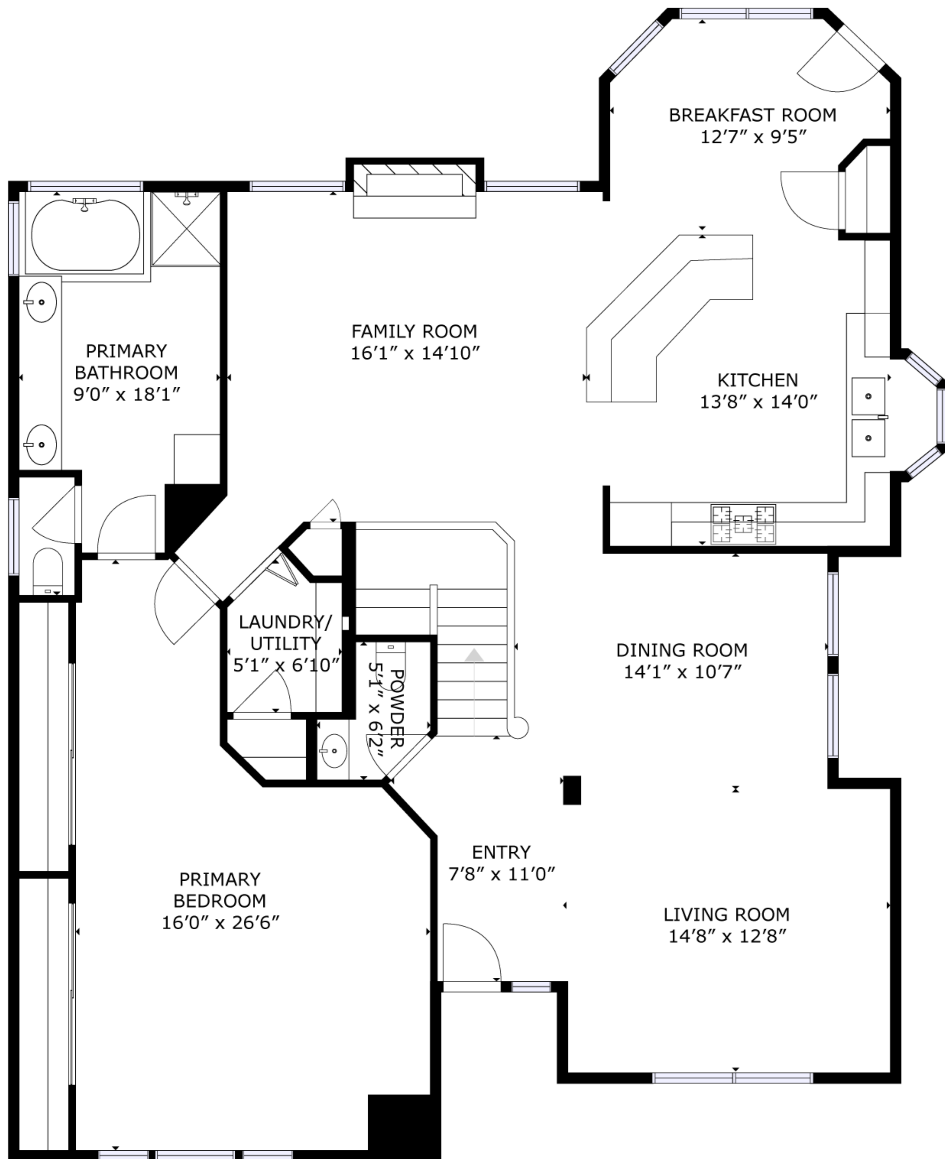
FLOOR 1
