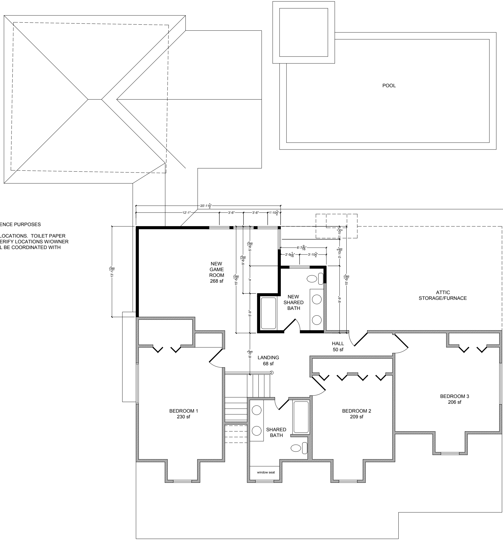
1/4"-1'-0" 1 Second Floor Plan
