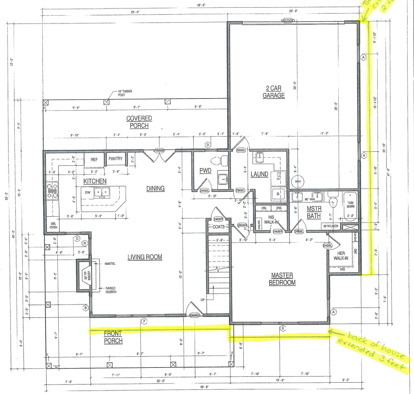
① FIRST FLOOR - PLAN 1/4" = 1'-0"
