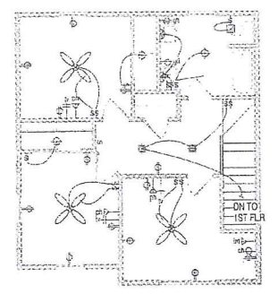
④ SECOND FLOOR - ELECTRICAL PLAN 1/8" = 1'-0"
