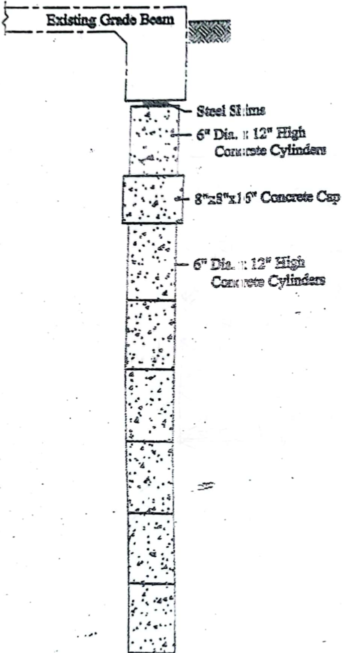
Cutaway View
