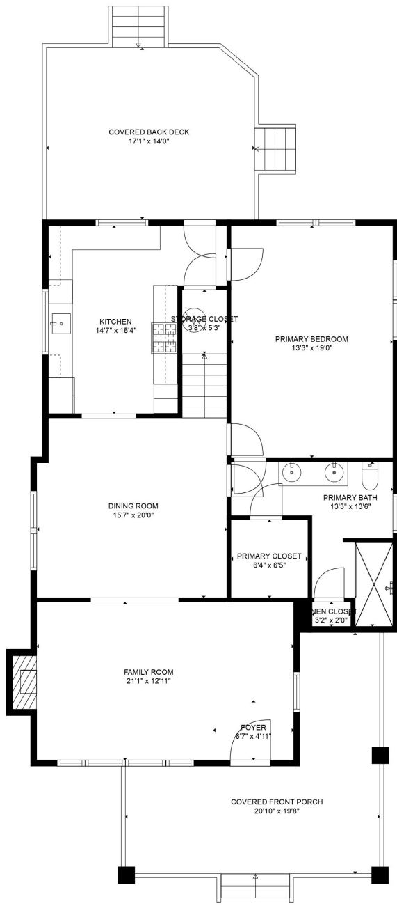
FLOOR 1
