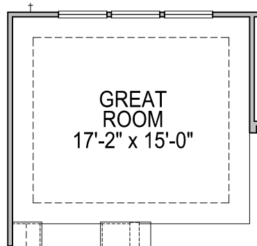
FIRST FLOOR PLAN OPT. #0714 GREAT ROOM COFFER
