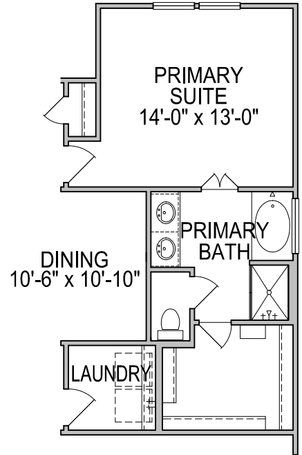
FIRST FLOOR PLAN OPT. #0751 PRIMARY BATH TUB
