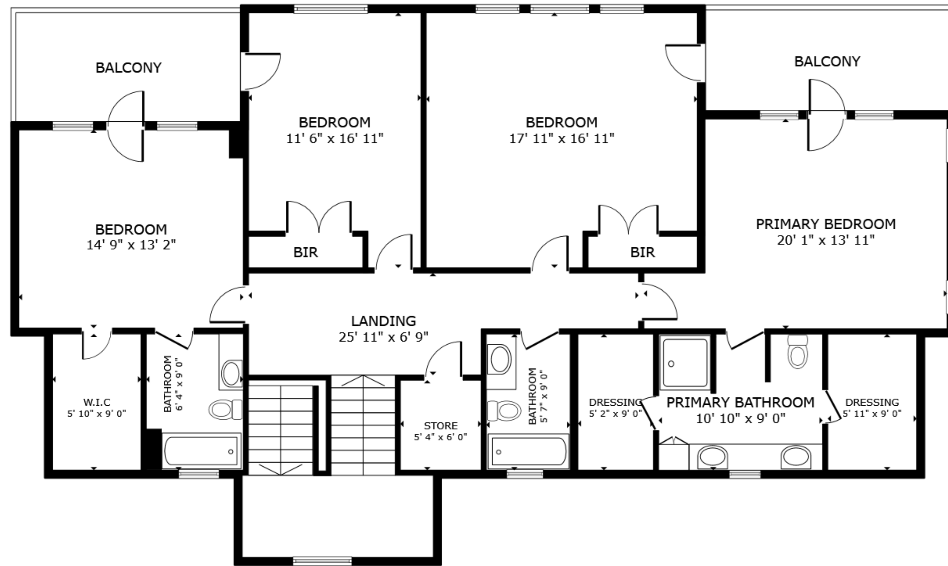
FLOOR 3
