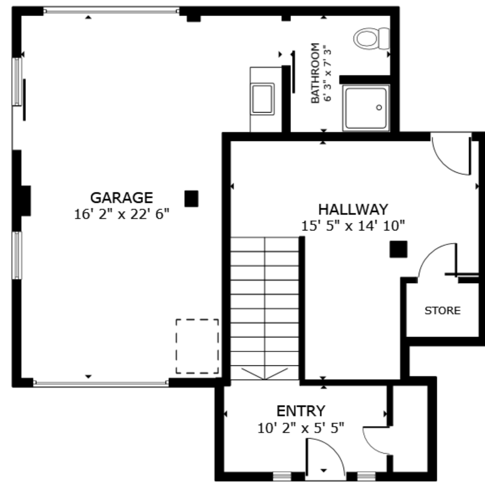
FLOOR 1
