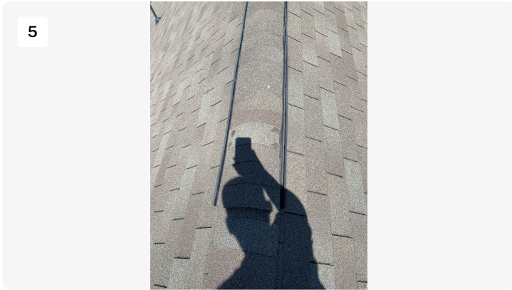
Lapped shingles over ridge vent
