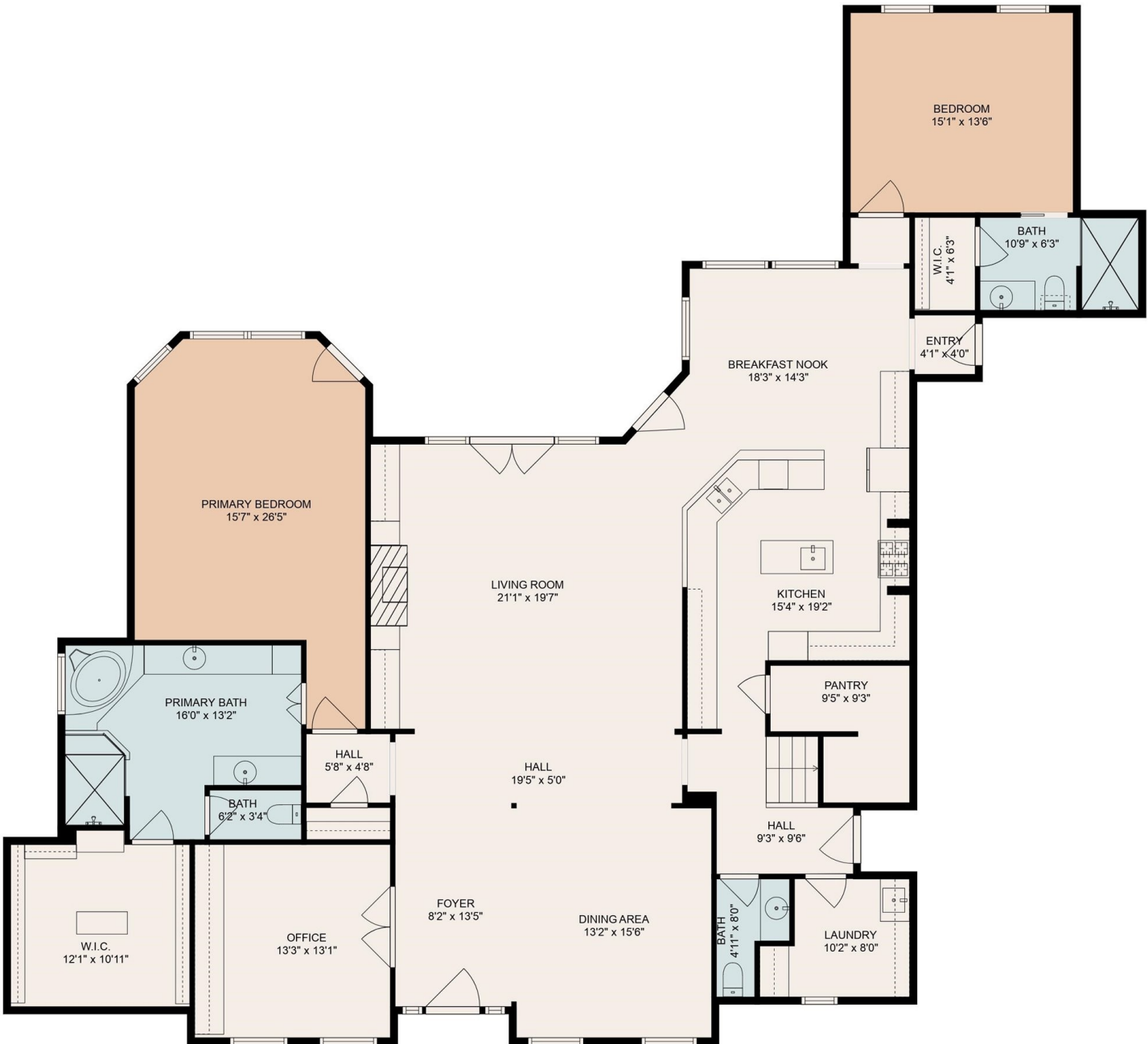
FLOOR 1
