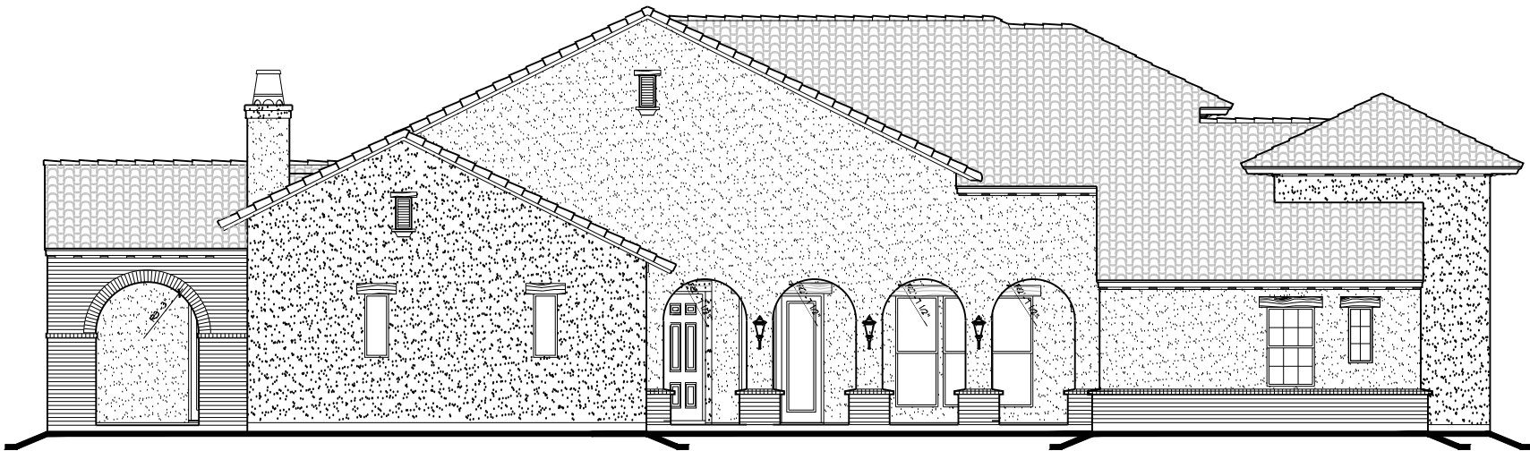
LEFT ELEVATION
