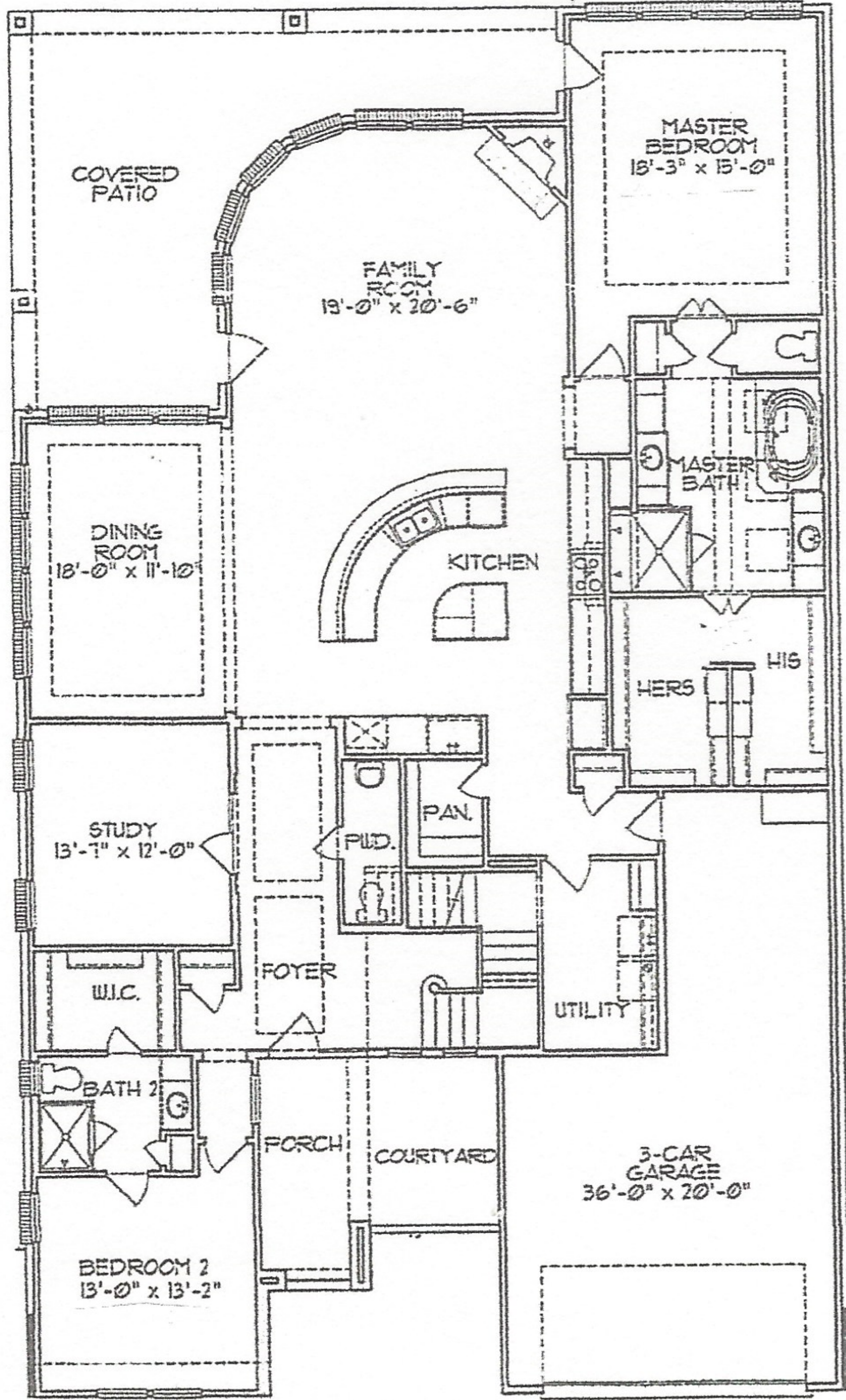
FIRST FLOOR
