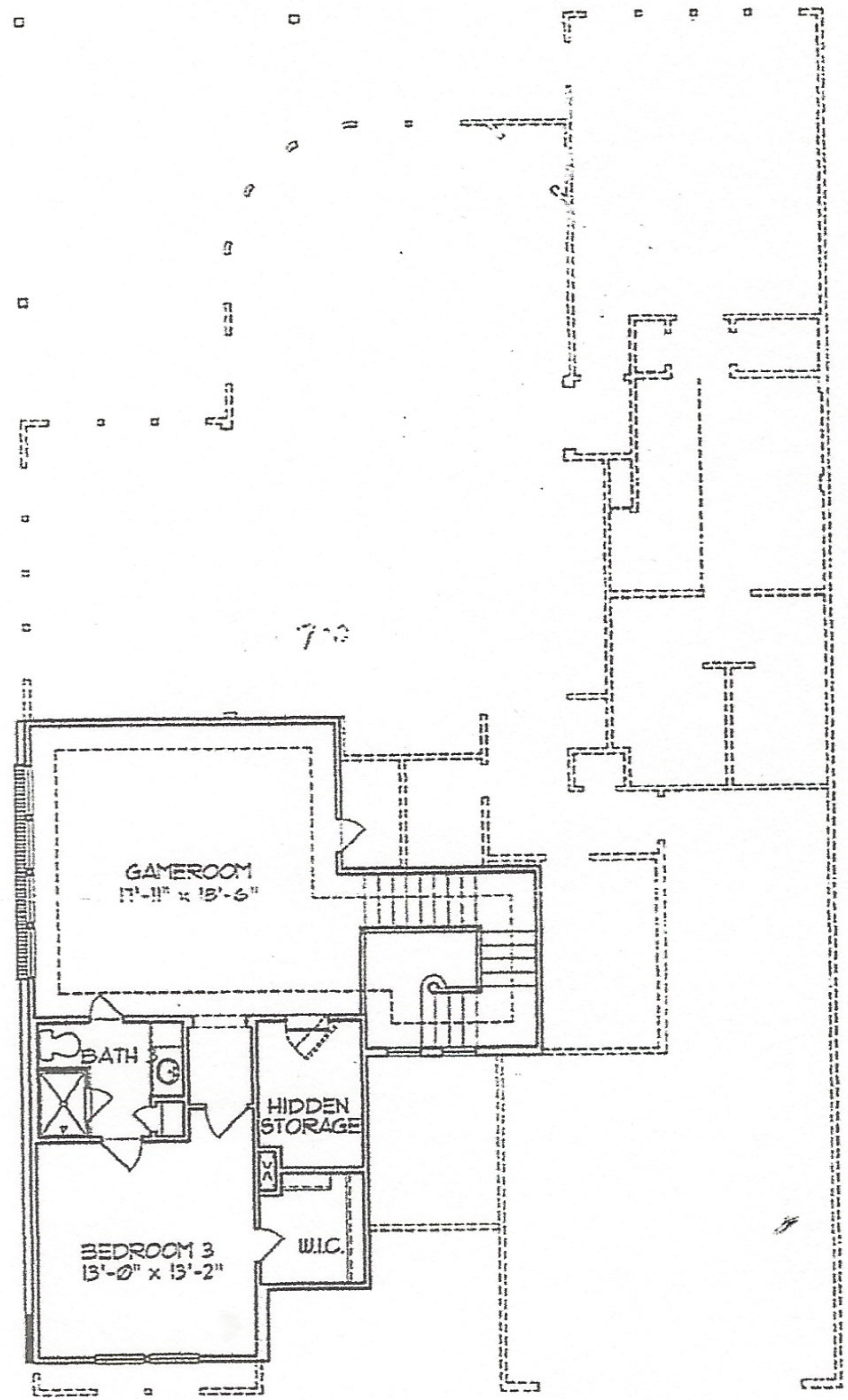
SECOND FLOOR
