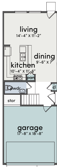
FIRST FLOOR
