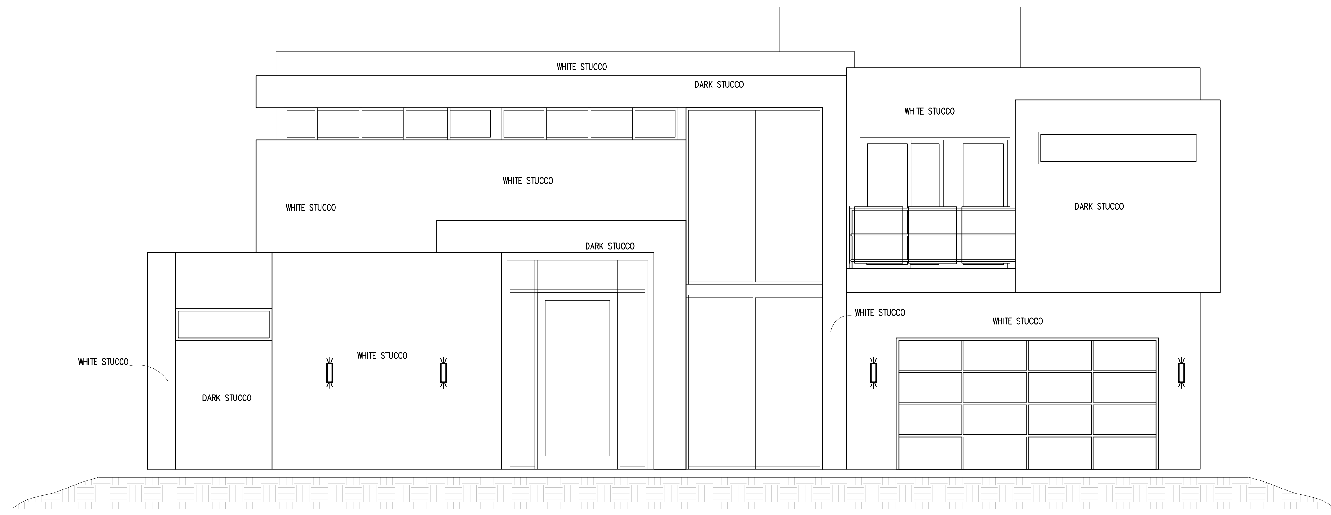
FRONT ELEVATION
