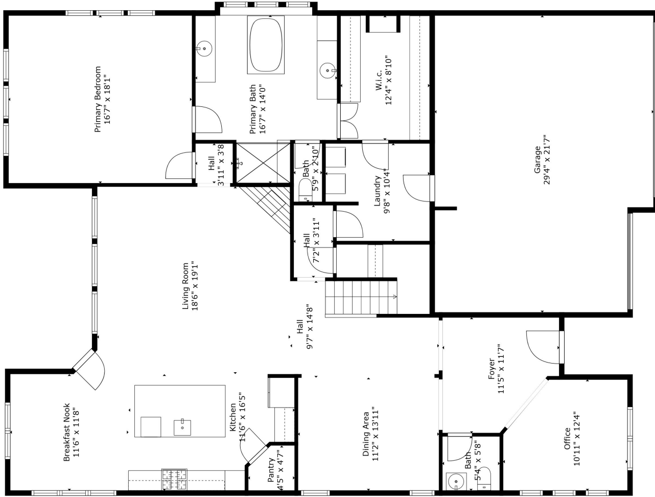
Floor 1
