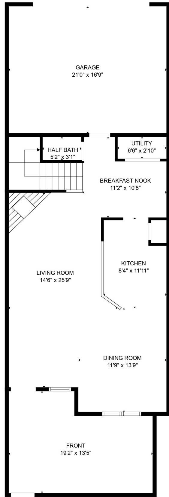
FLOOR 1
