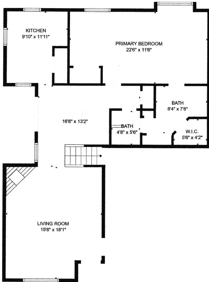
FLOOR 1
