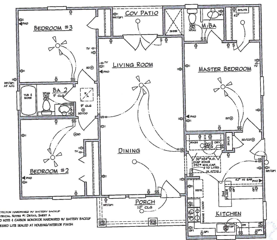
ELECTRICAL PLAN SCALE 1/4" = 1'-0"
