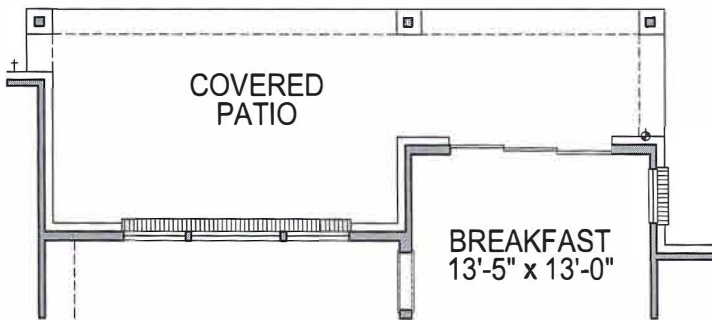
FIRST FLOOR PLAN OPT. #0788 EXT. COVERED PATIO W/ SLIDERS @ BREAKFAST
