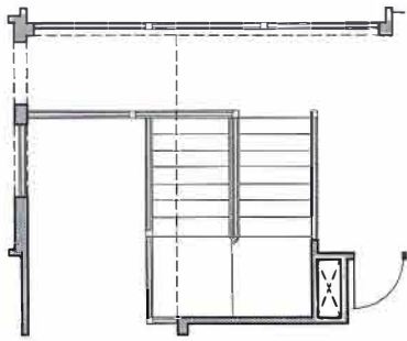
SECOND FLOOR PLAN OPT. #0134 STRAIGHT STAIRS
