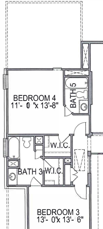
SECOND FLOOR PLAN OPT. #0567 BATH 5
