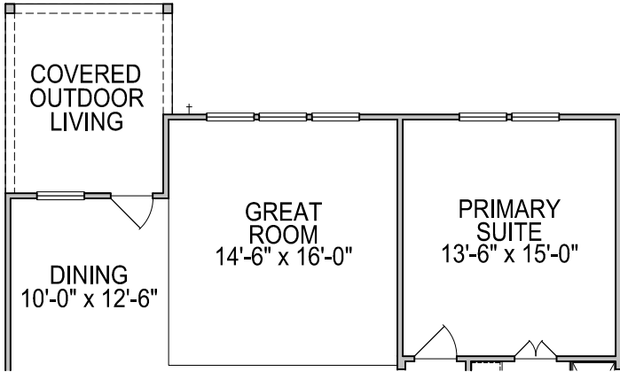
FIRST FLOOR PLAN OPT. #0105 COVERED OUTDOOR LIVING
