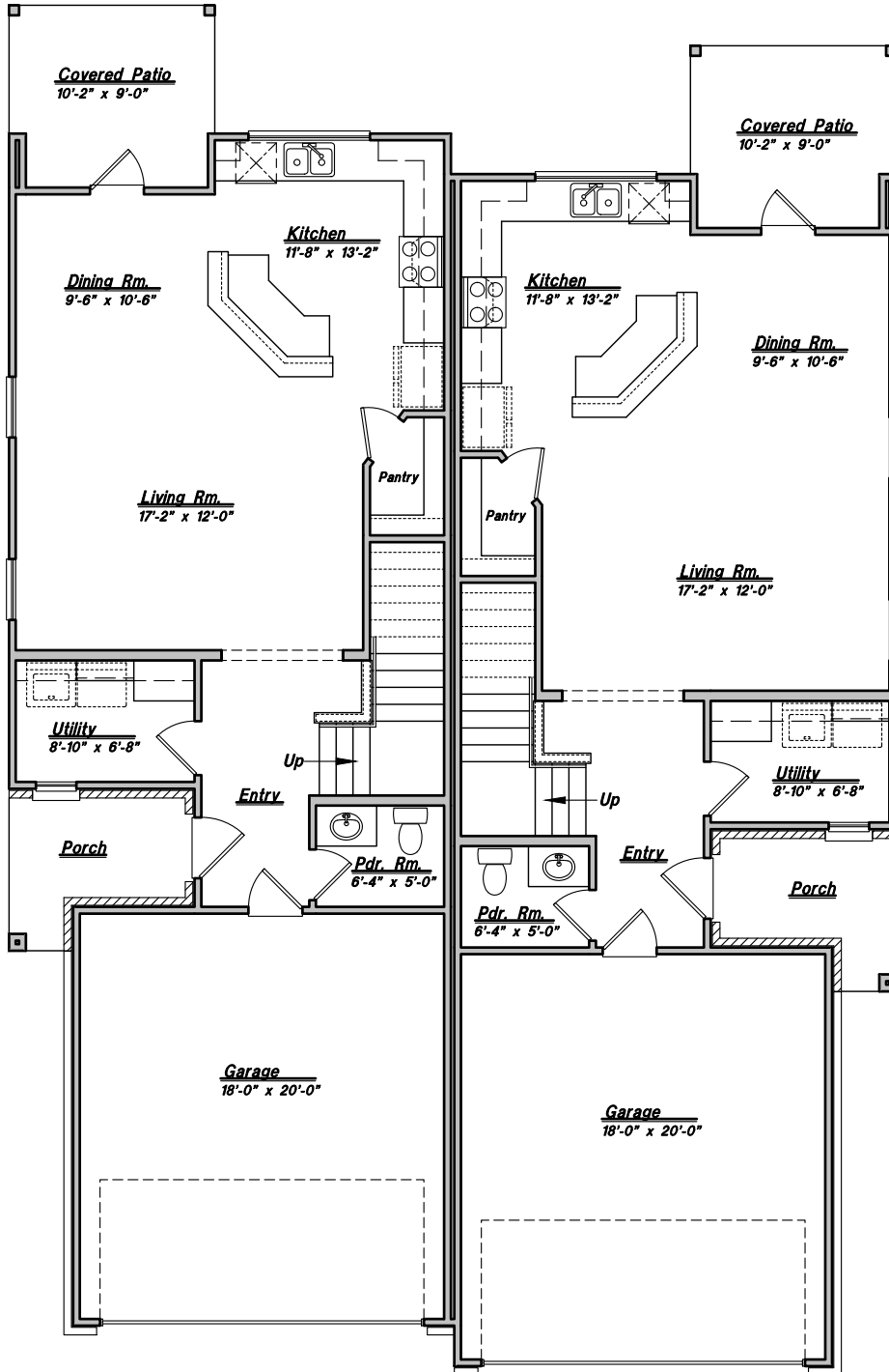
FIRST FLOOR PLAN Plan 1580 'ELOISA'
