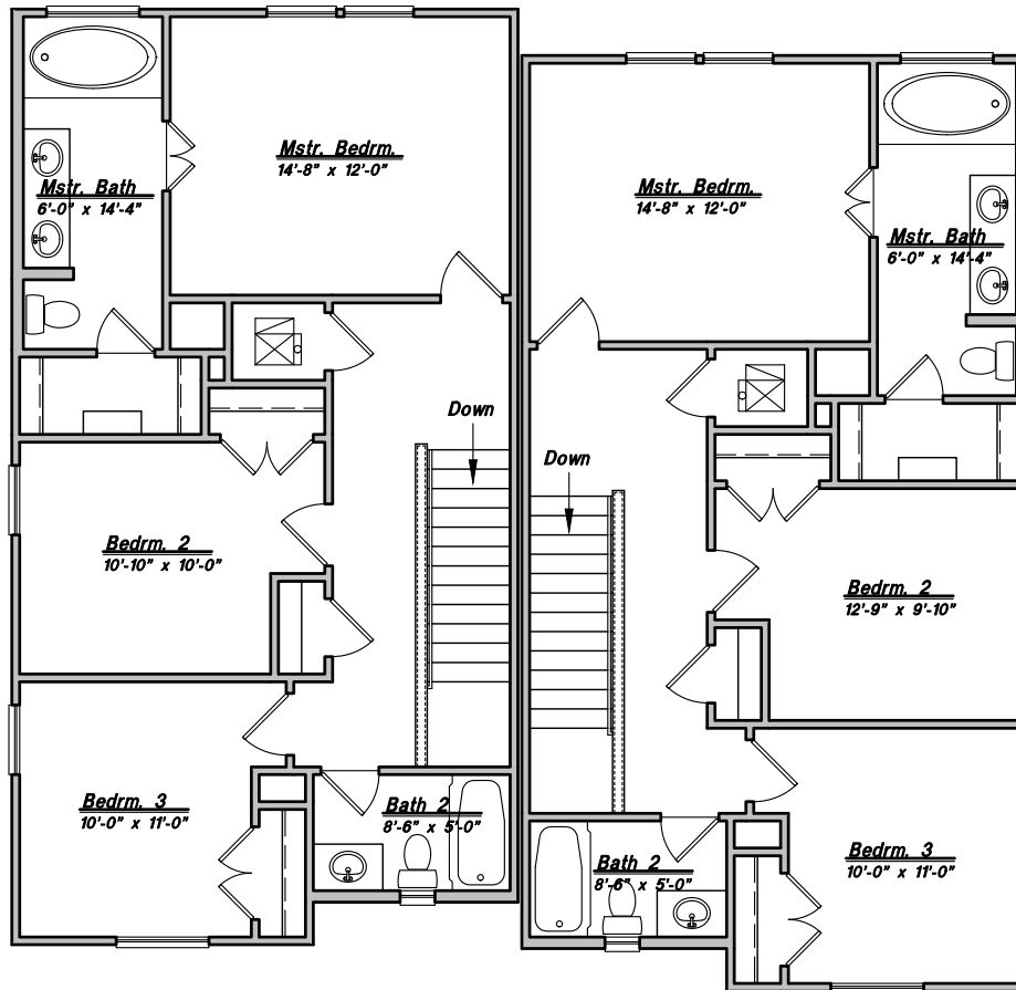
SECOND FLOOR PLAN Plan 1580 'ELOISA'
