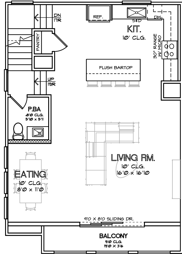
SECOND FLOOR PLAN PLAN 1963
