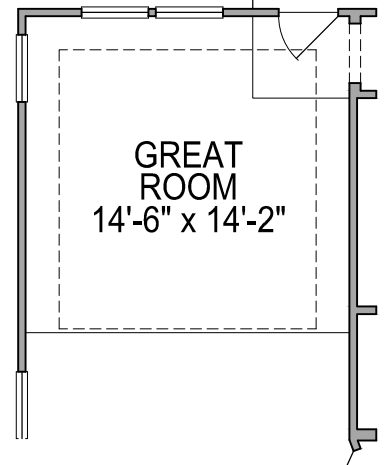
FIRST FLOOR PLAN OPT. #0714 GREAT ROOM COFFER
