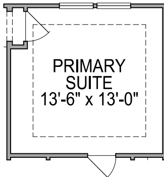
FIRST FLOOR PLAN OPT. #0668 PRIMARY SUITE COFFER
