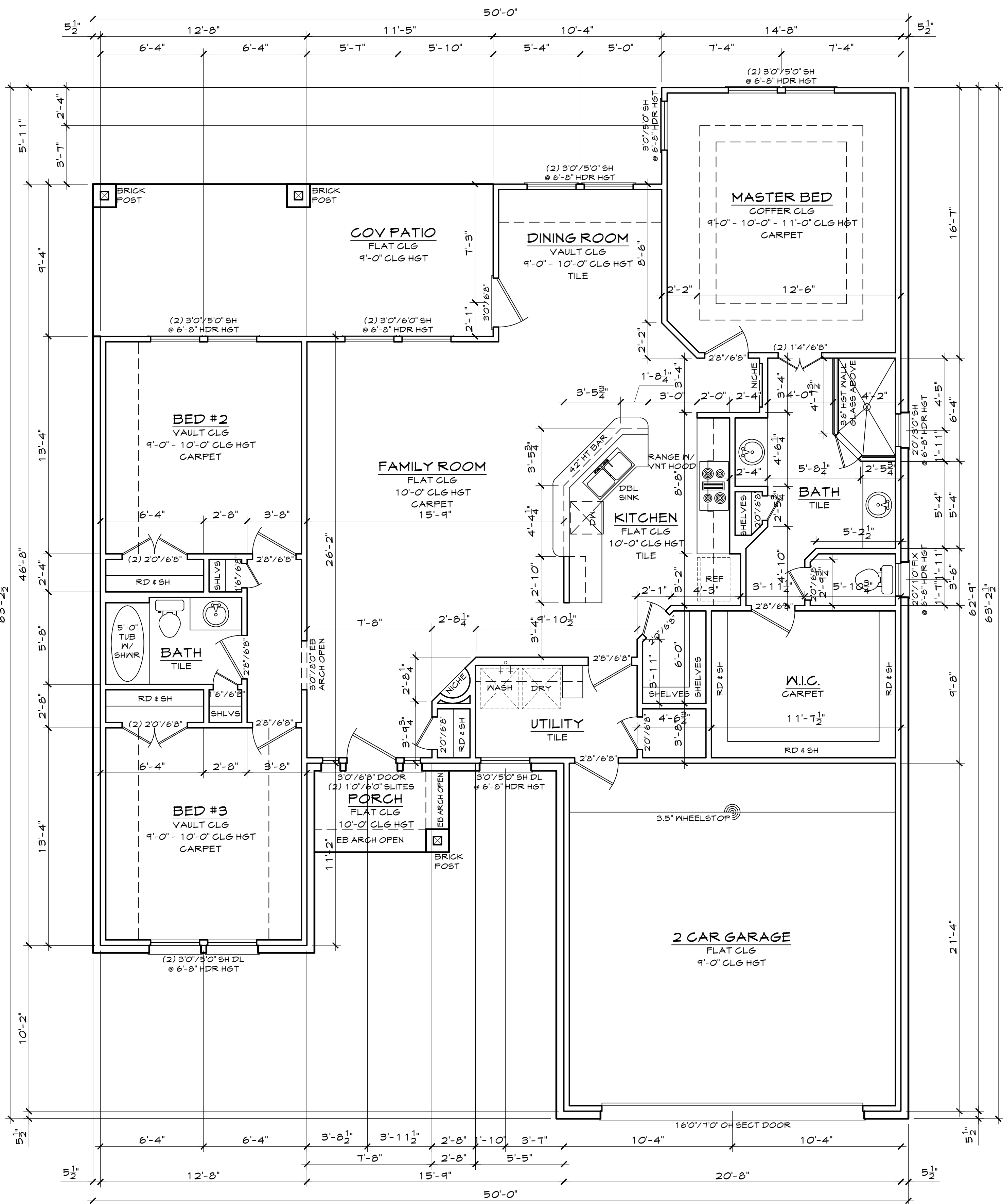
1 FLOOR PLAN SCALE: 1/4" = 1'
