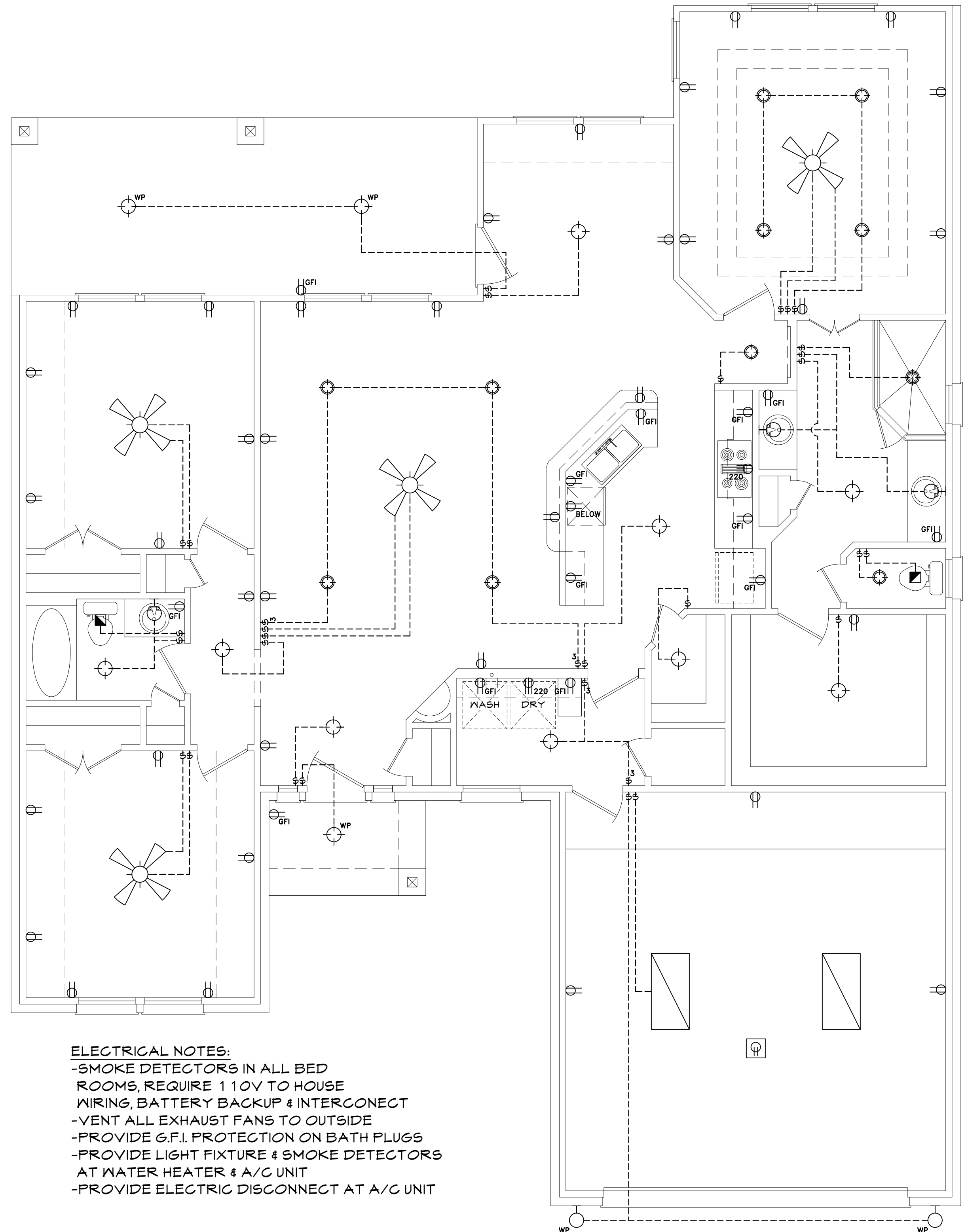
2 ELECTRICAL SCALE: 1/4" = 1'
