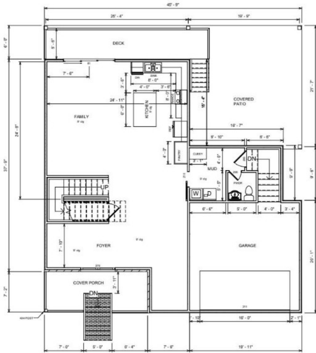
① Proposed 1st Floor 1/8" = 1'-0"
