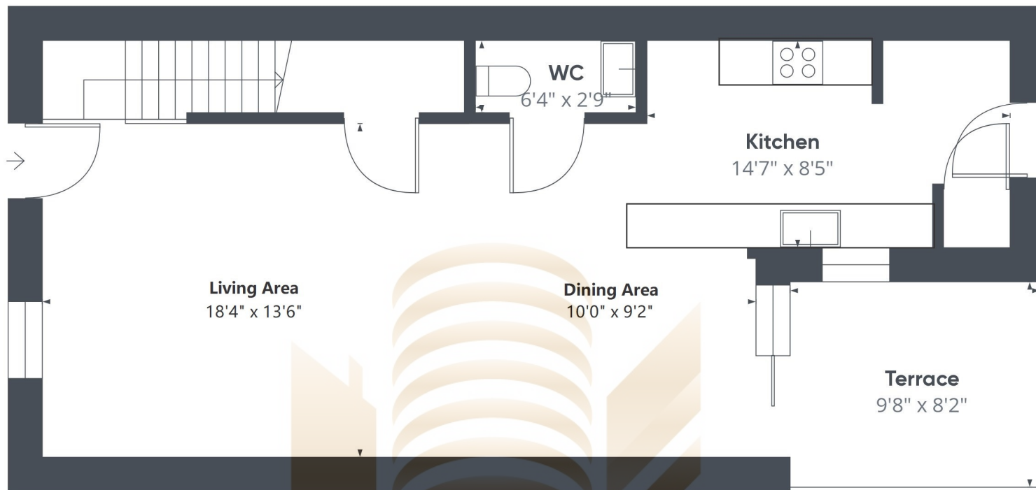
Floor 1
