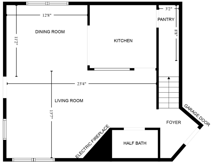
FLOOR 1
