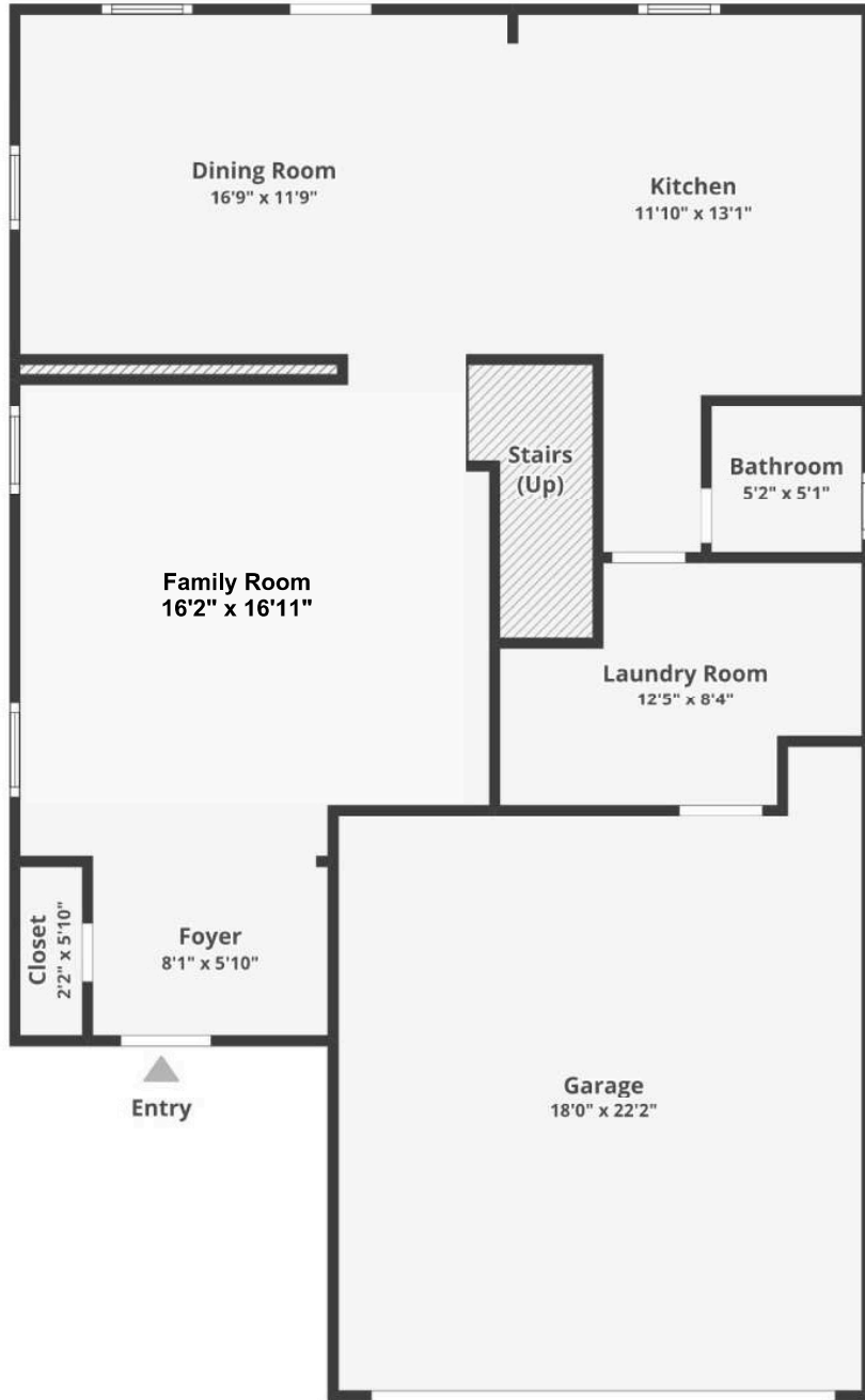
FLOOR 1
