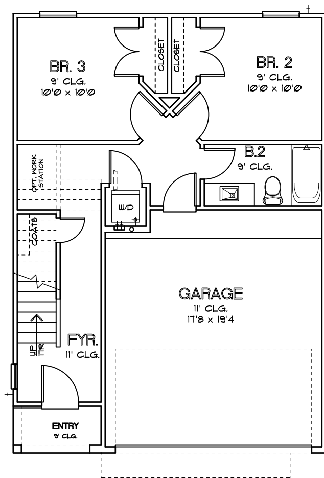
FIRST FLOOR PLAN PLAN A1422 L
