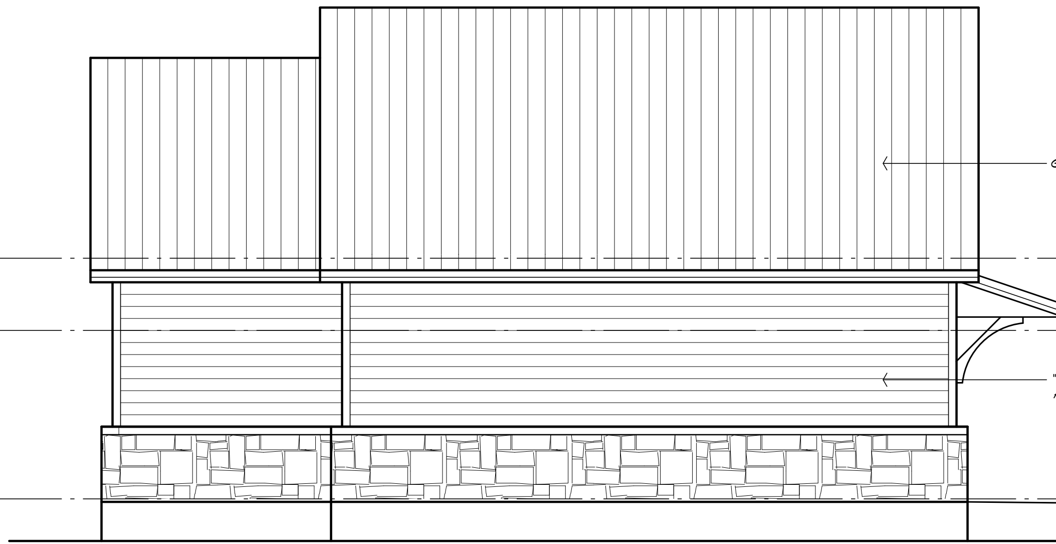
3 CLUB HOUSE BACK ELEVATION 1/4" = 1'-0"
