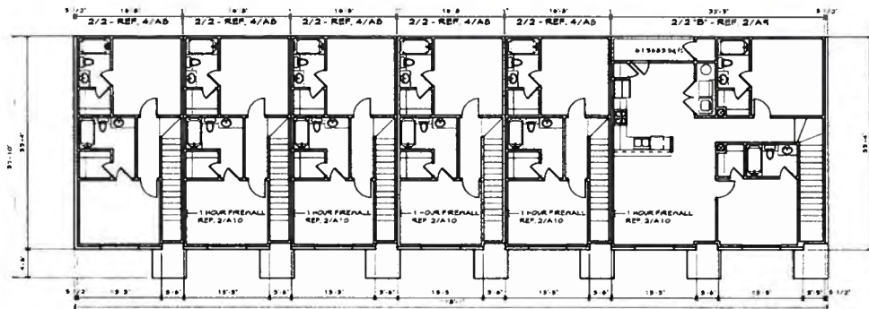
② BLDG. F - 2nd FLOOR PLAN PHASE 3 1/8" = 1'-0"
