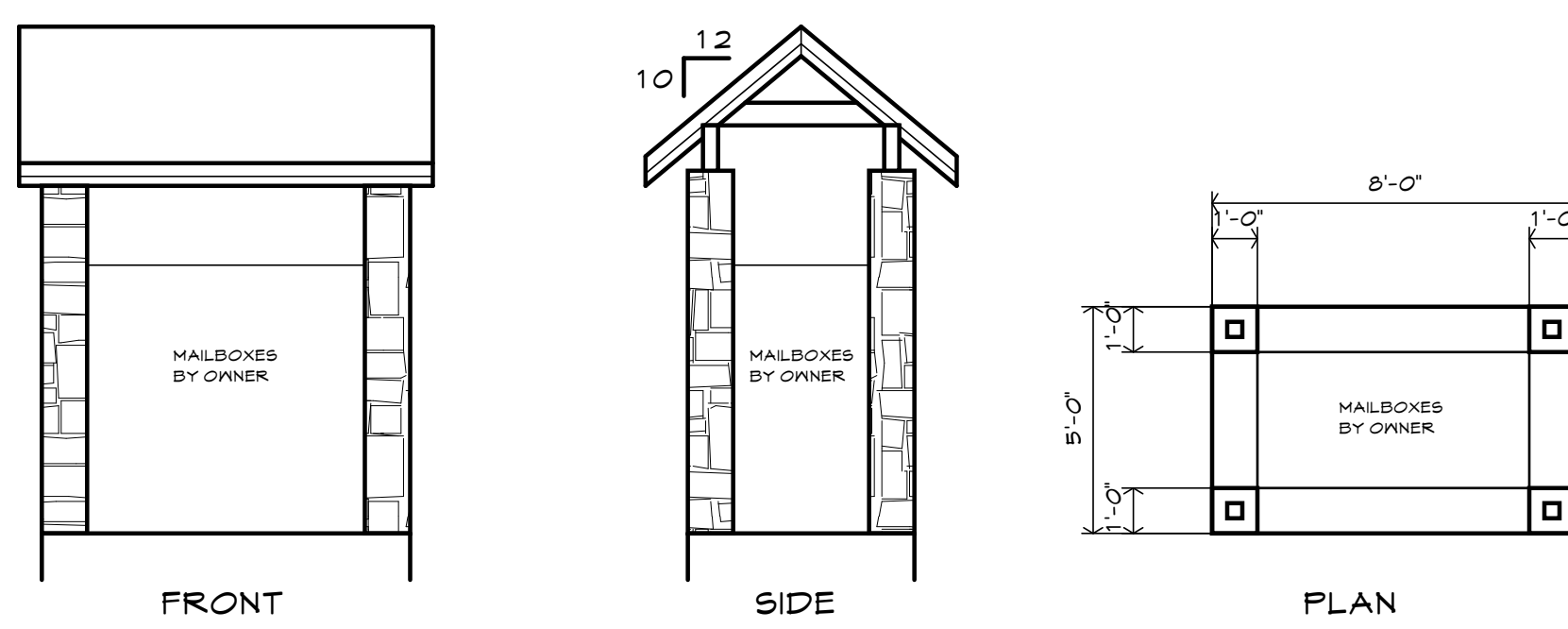
7 MAIL BOX STRUCTURE 1/4" = 1'-0"
