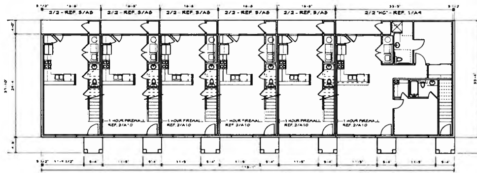
② BLDG. F - 2nd FLOOR PLAN PHASE 3 1/8" = 1'-0"
