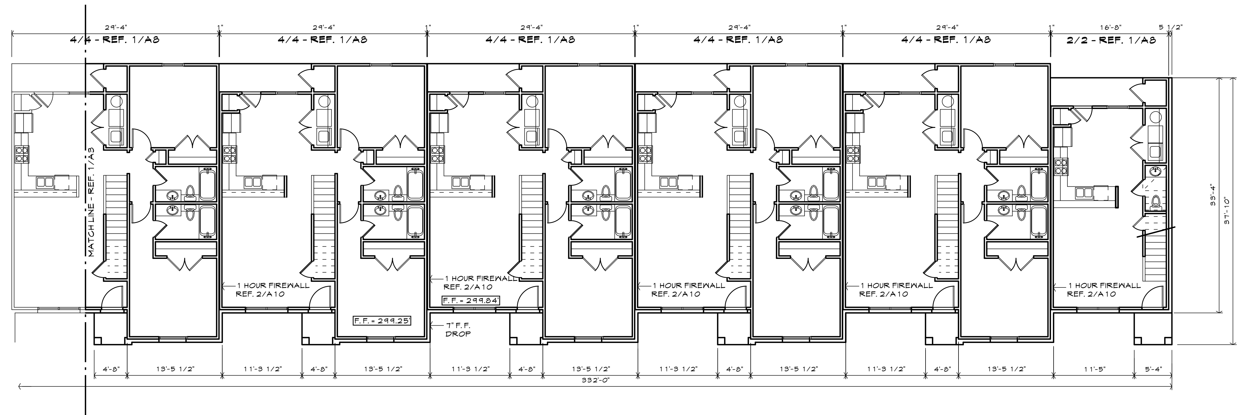
② BLDG. E - 1st FLOOR PLAN (RIGHT) PHASE 1 1/8" = 1'-0"
