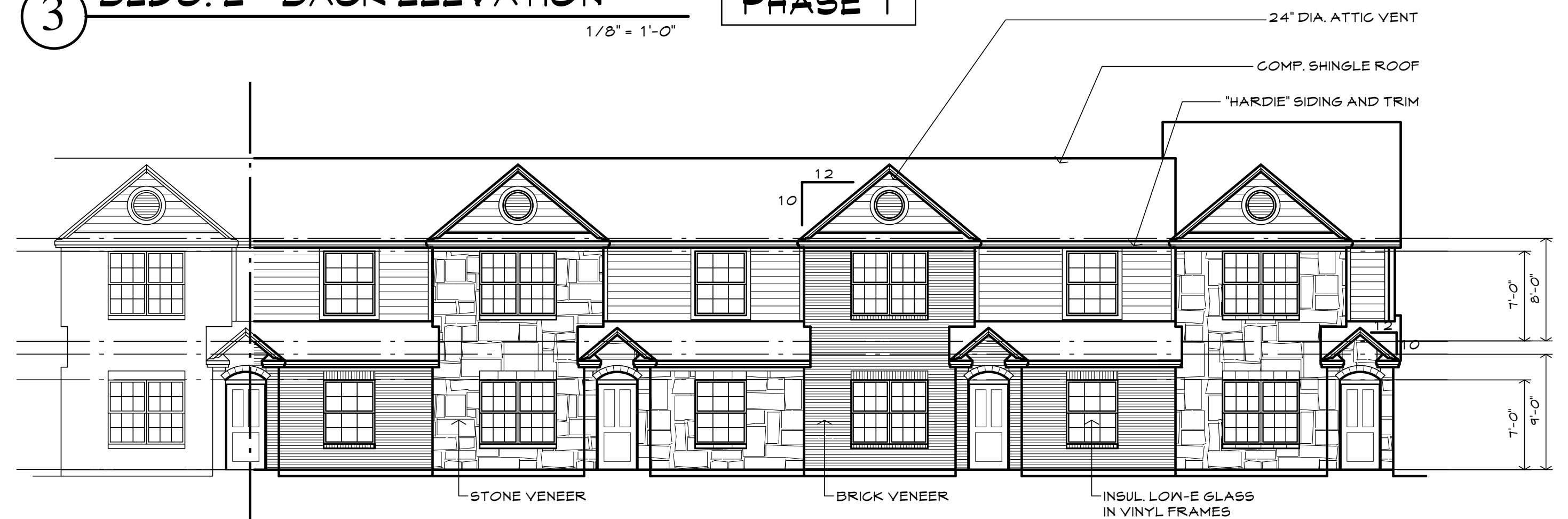
2 BLDG. E - FRONT ELEVATION 1/8" = 1'-0"
