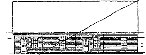
4 BLDG. C - BACK ELEVATION 1/8" = 1'-0"
