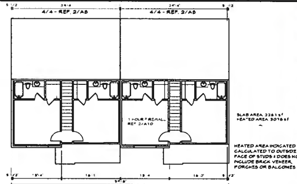
4 BLDG. C - 2nd FLOOR PLAN
