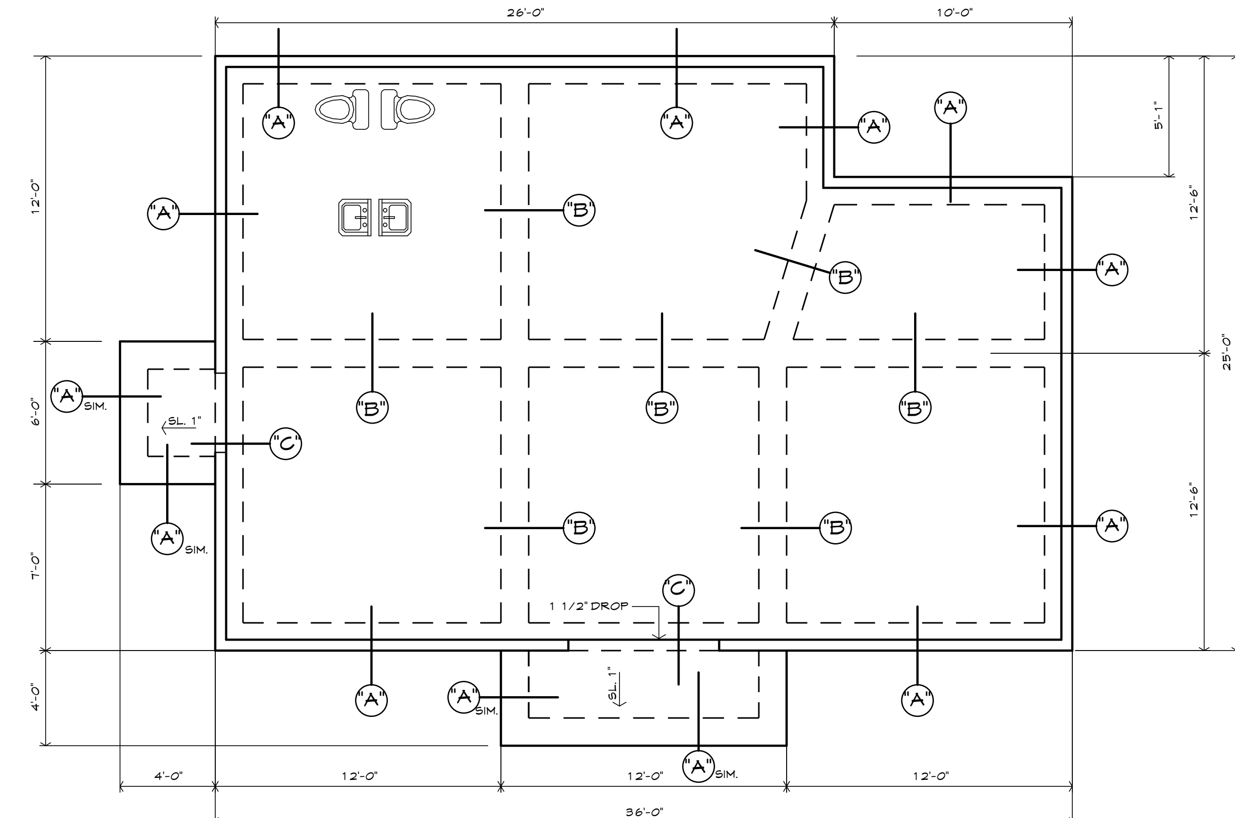
1 FOUNDATION PLAN CLUB HOUSE PHASE 1 1/4" = 1'-0"
