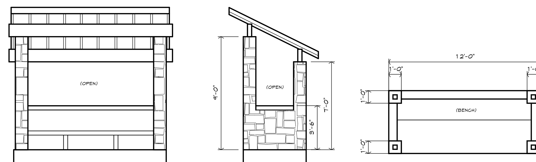
6 BUS STOP STRUCTURE 1/4" = 1'-0"
