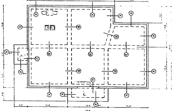
1 FOUNDATION PLAN CLUB HOUSE PHASE 1 1/4" = 1'-0"
