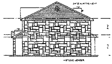
6 BLDG. E - RIGHT SIDE ELEV. PHASE 1
