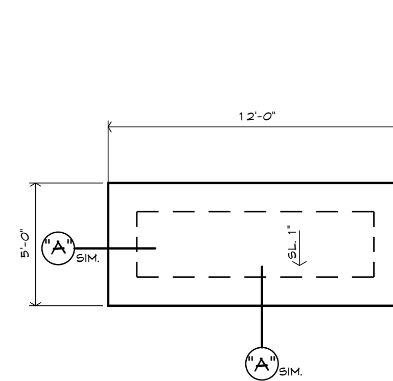
3 FOUND. PLAN MAILBOX 1/4" = 1'-0"
