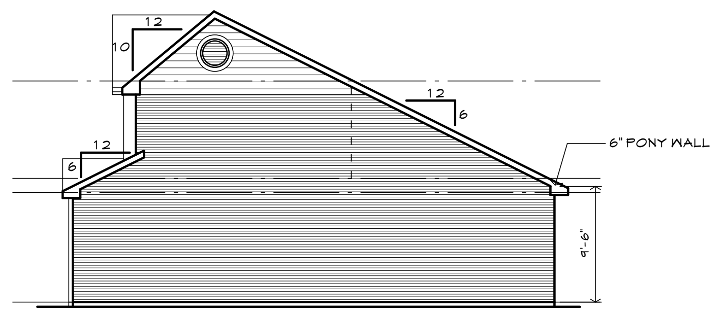
5 BLDG. A, B & C - RIGHT SIDE ELEV. 1/8" = 1'-0" BLDG. A - PHASE 1
