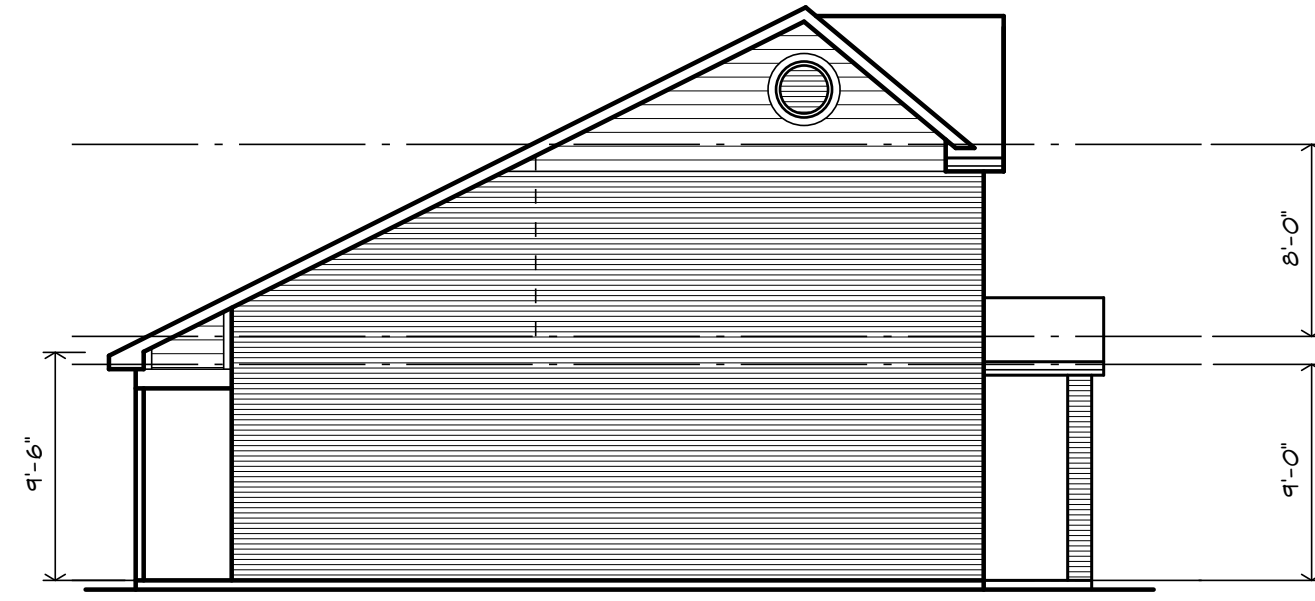
6 BLDG. A, B & C - LEFT SIDE ELEV. 1/8" = 1'-0" BLDG. A - PHASE 1
