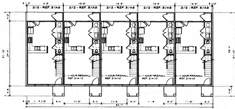
④ BLDG. G - 2nd FLOOR PLAN PHASE 3 1/8" = 1'-0"
