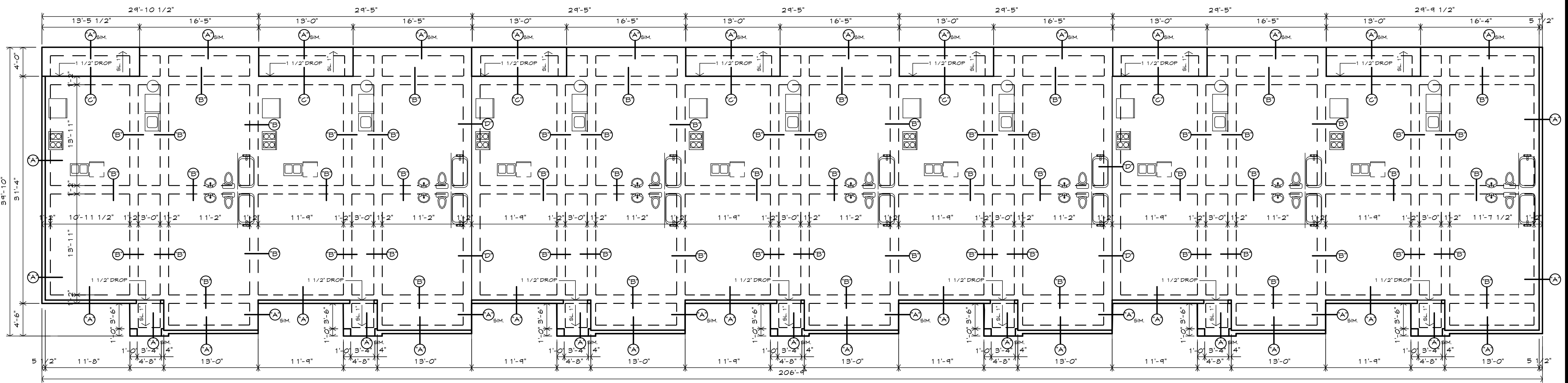
3 FOUNDATION DETAILS NOTE: GRADE BEAMS TO EXTEND MIN. 1'-0" INTO UNDISTURBED SOIL 3/4" = 1'-0"
