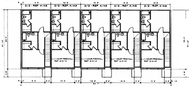
④ BLDG. G - 2nd FLOOR PLAN PHASE 3 1/8" = 1'-0"
