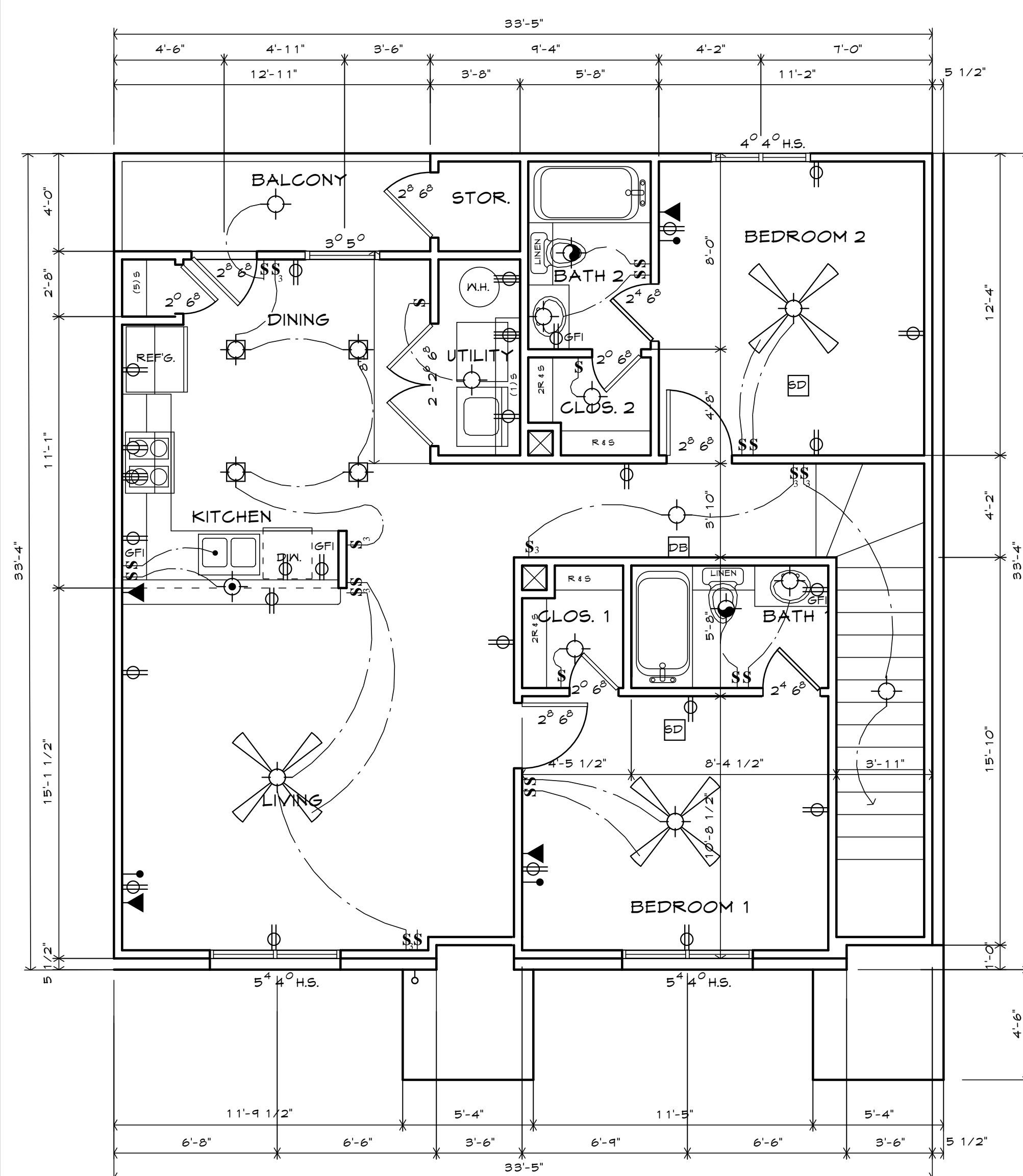
④ 2nd FLOOR PLAN 2-2 "B" Heated Area: 1029 s.f. 1/4" = 1'-0"
