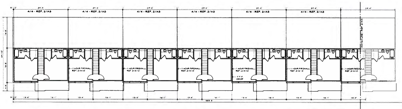
1 BLDG. D - 2nd FLOOR PLAN (LEFT) PHASE 3 1/8" = 1'-0"
