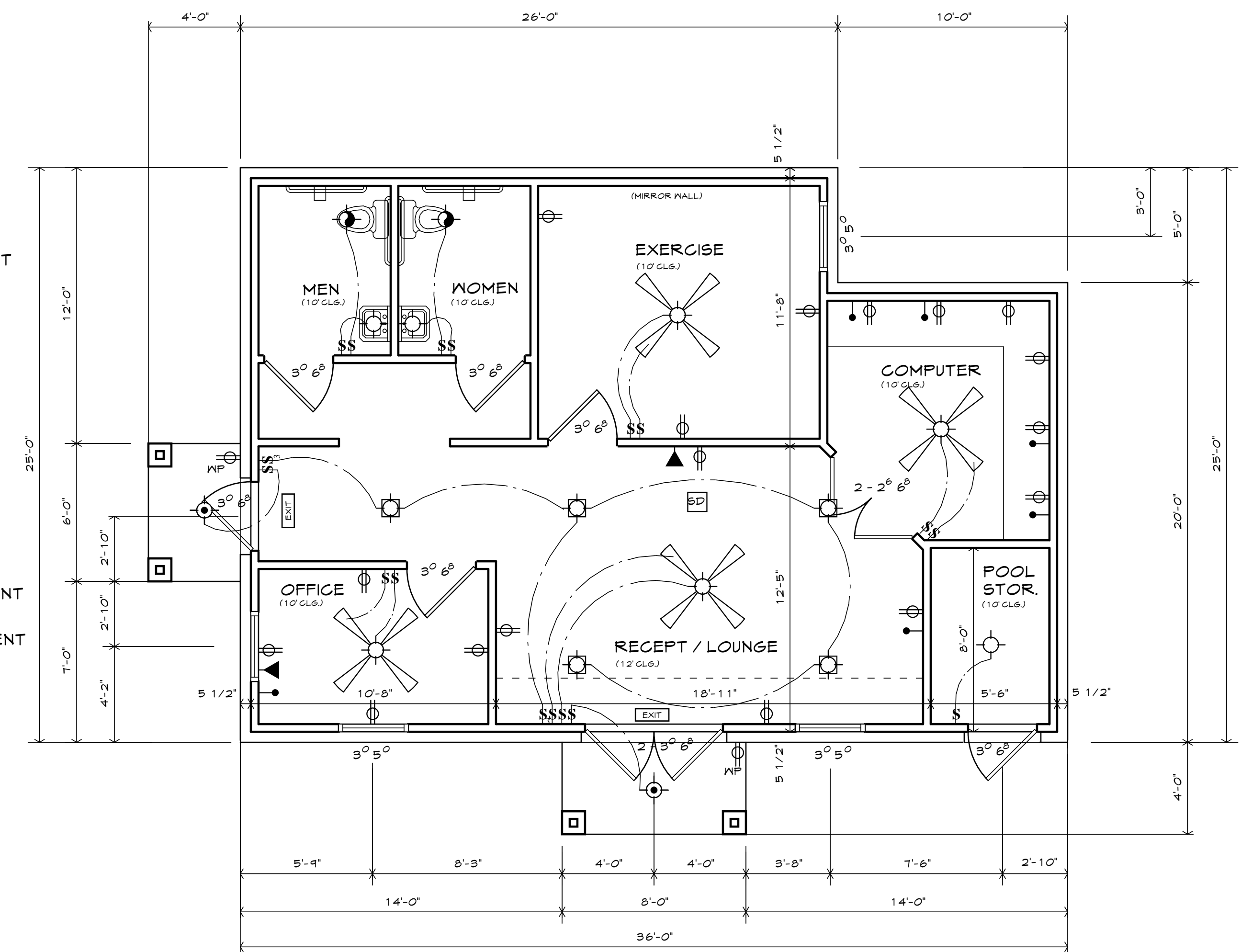
1 CLUB HOUSE FLOOR PLAN 1/4" = 1'-0" PHASE 1
