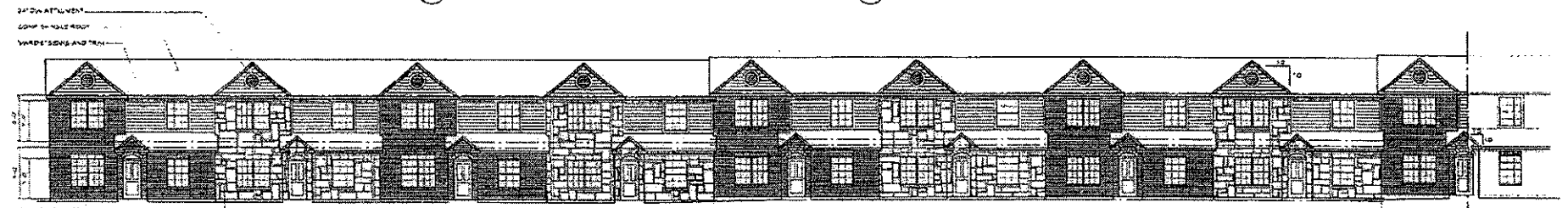
1 BLDG. E - FRONT ELEVATION PHASE 1
