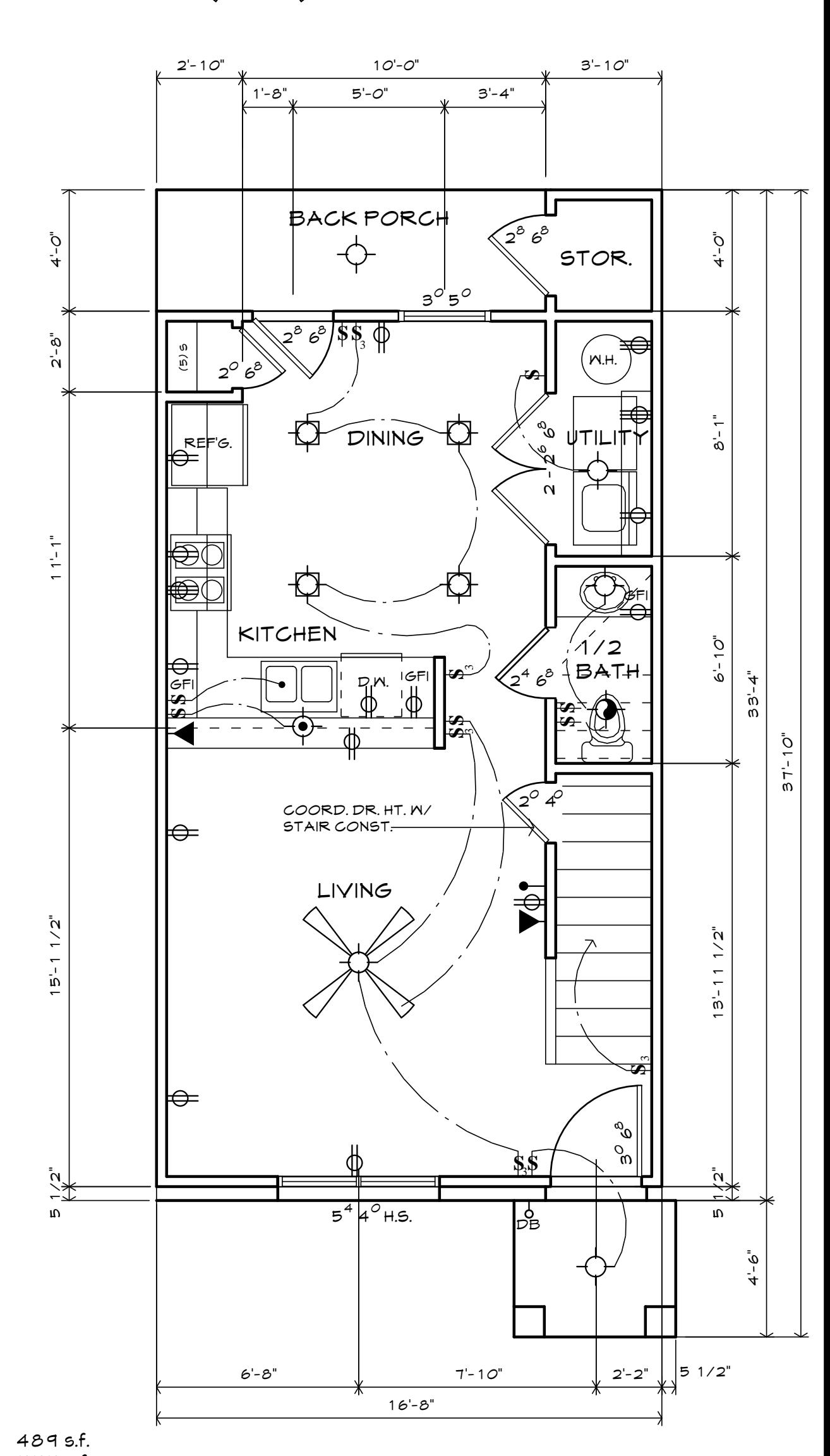
① 1st FLOOR PLAN 2-2 1/4" = 1'-0"
