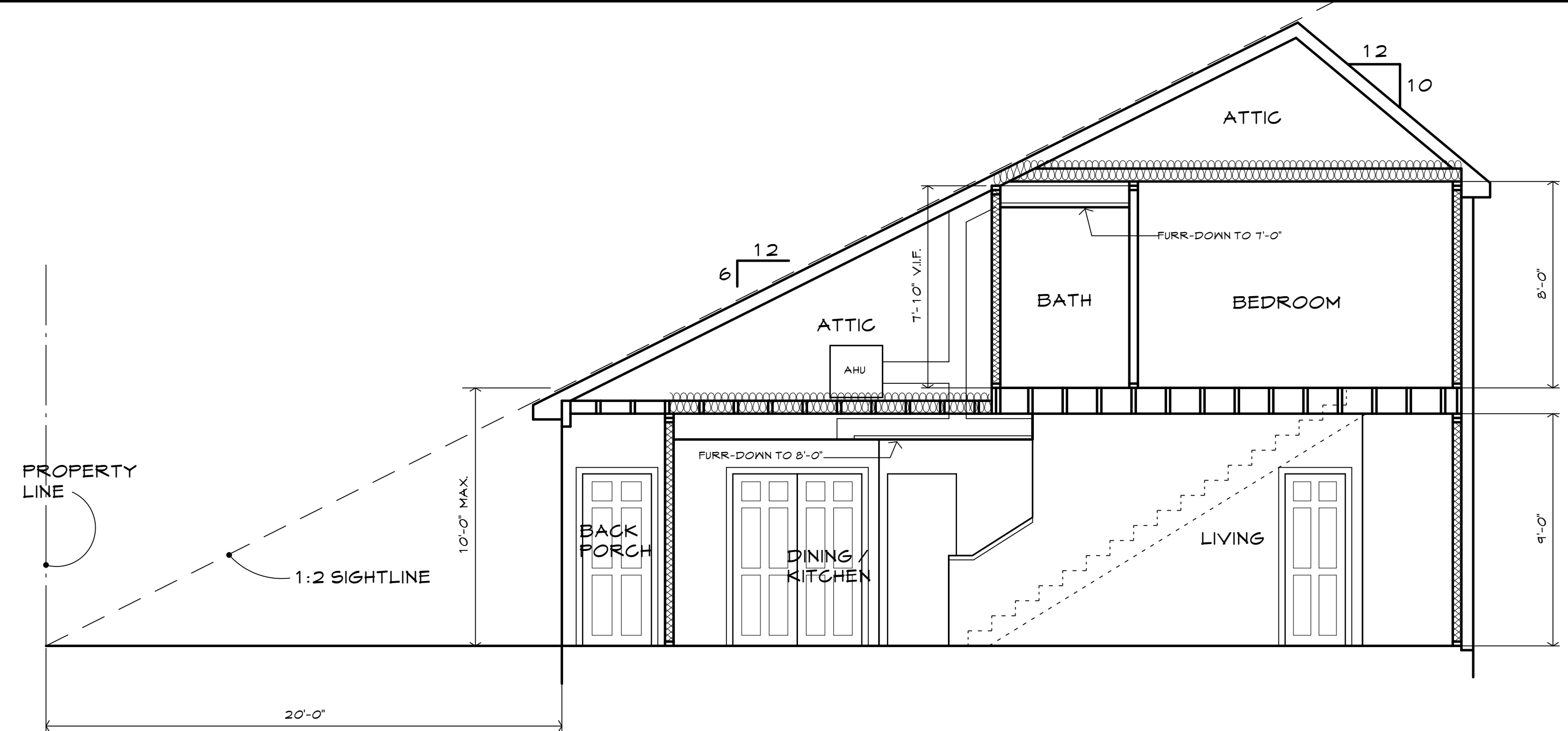
③ 4-4 SECTION 1/4" = 1'-0"
