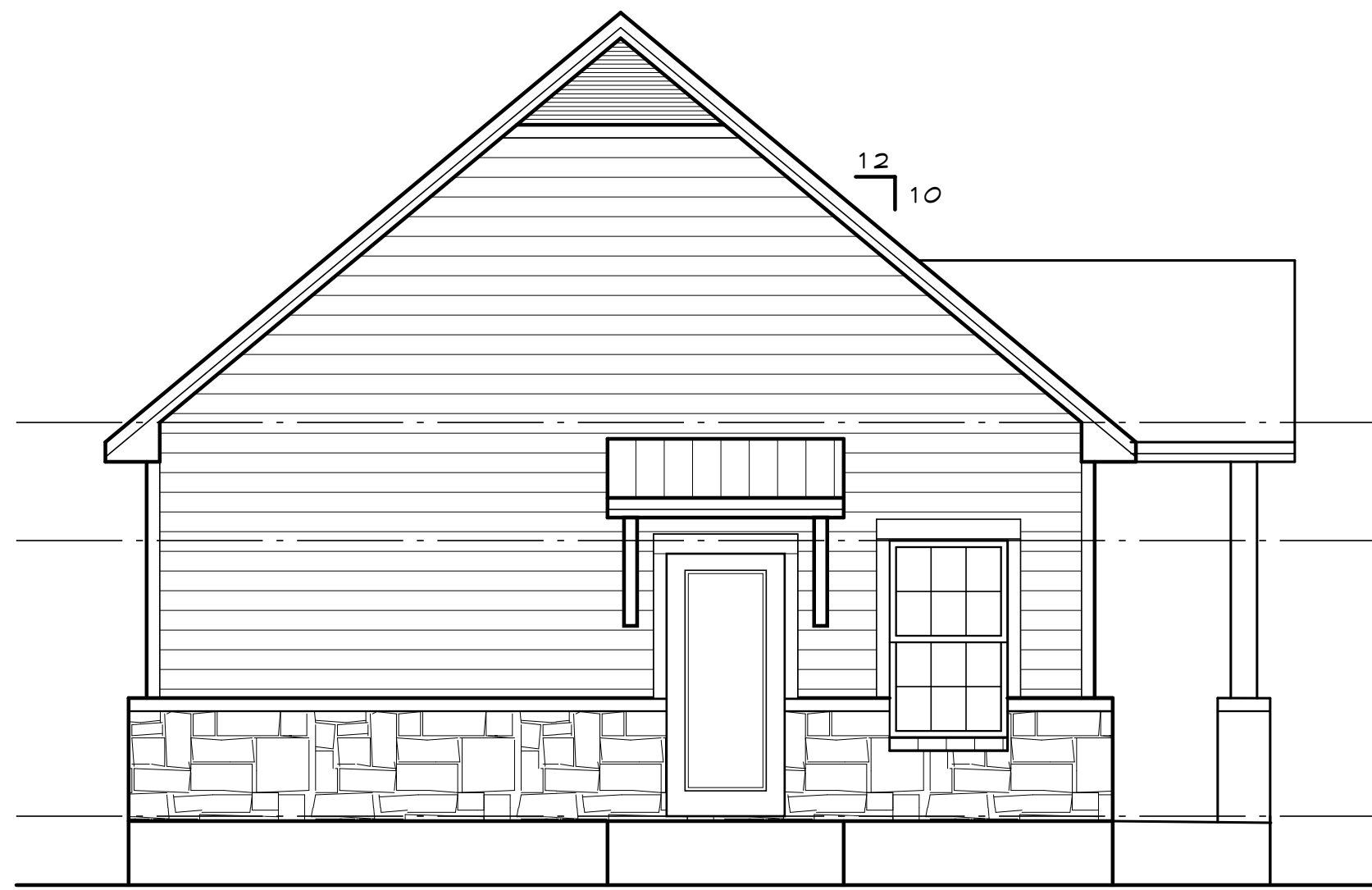
4 CLUB HOUSE SIDE ELEVATION 1/4" = 1'-0"
