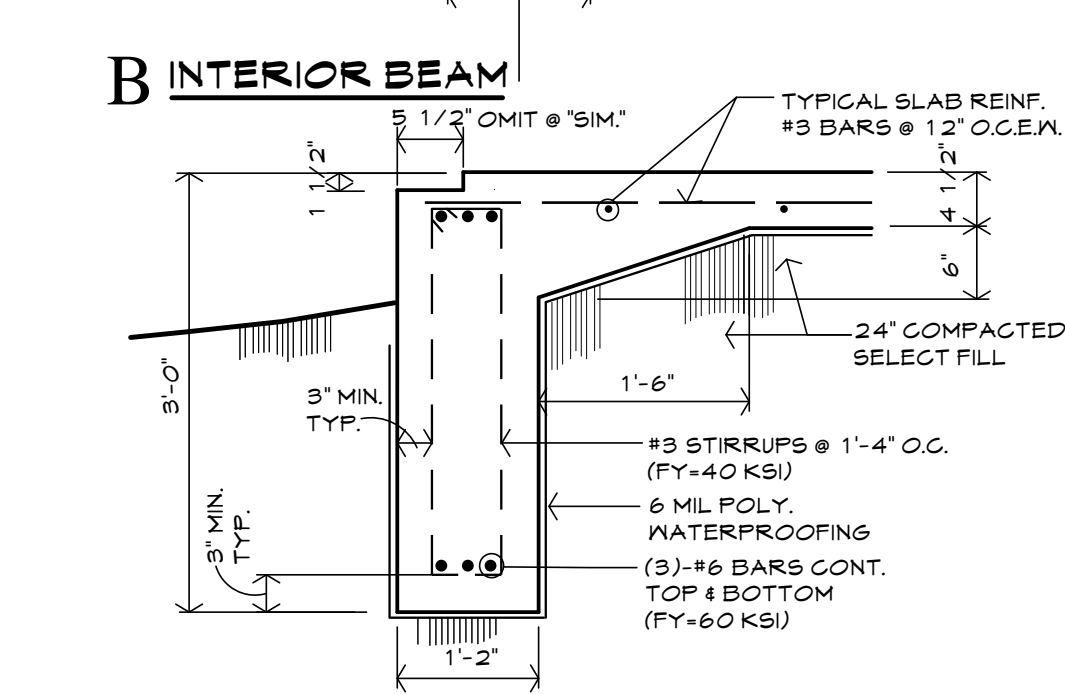
4 FOUNDATION DETAILS 3/4" = 1'-0"
