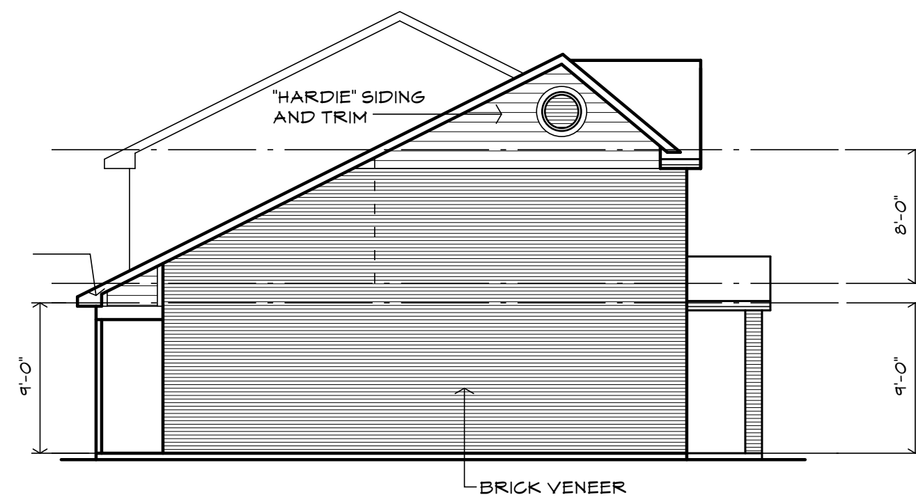
5 BLDG. E - LEFT SIDE ELEV. 1/8" = 1'-0"
