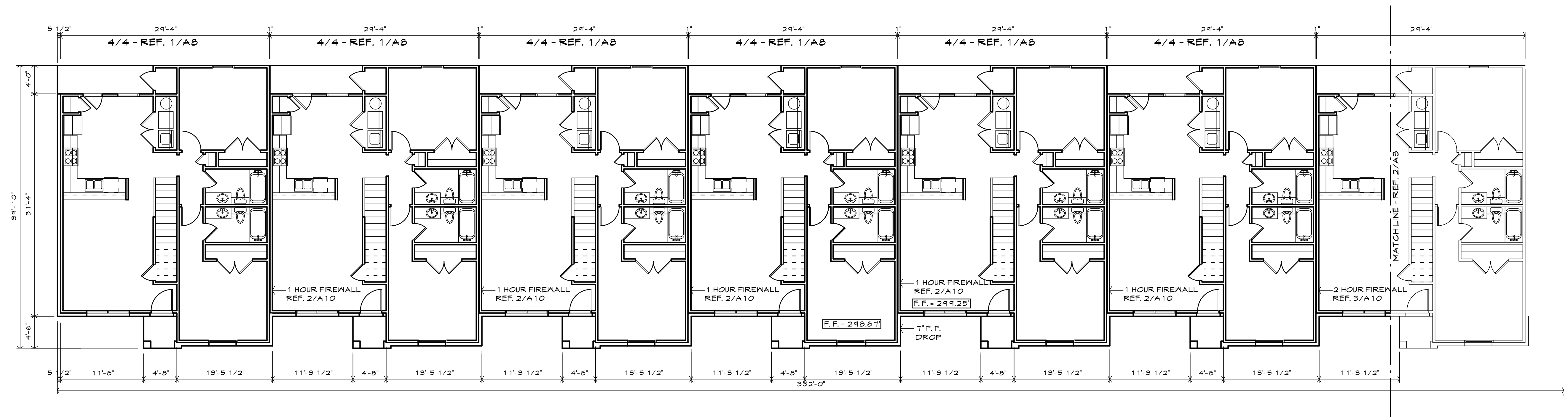
① BLDG. E - 1st FLOOR PLAN (LEFT) PHASE 2 1/8" = 1'-0"
