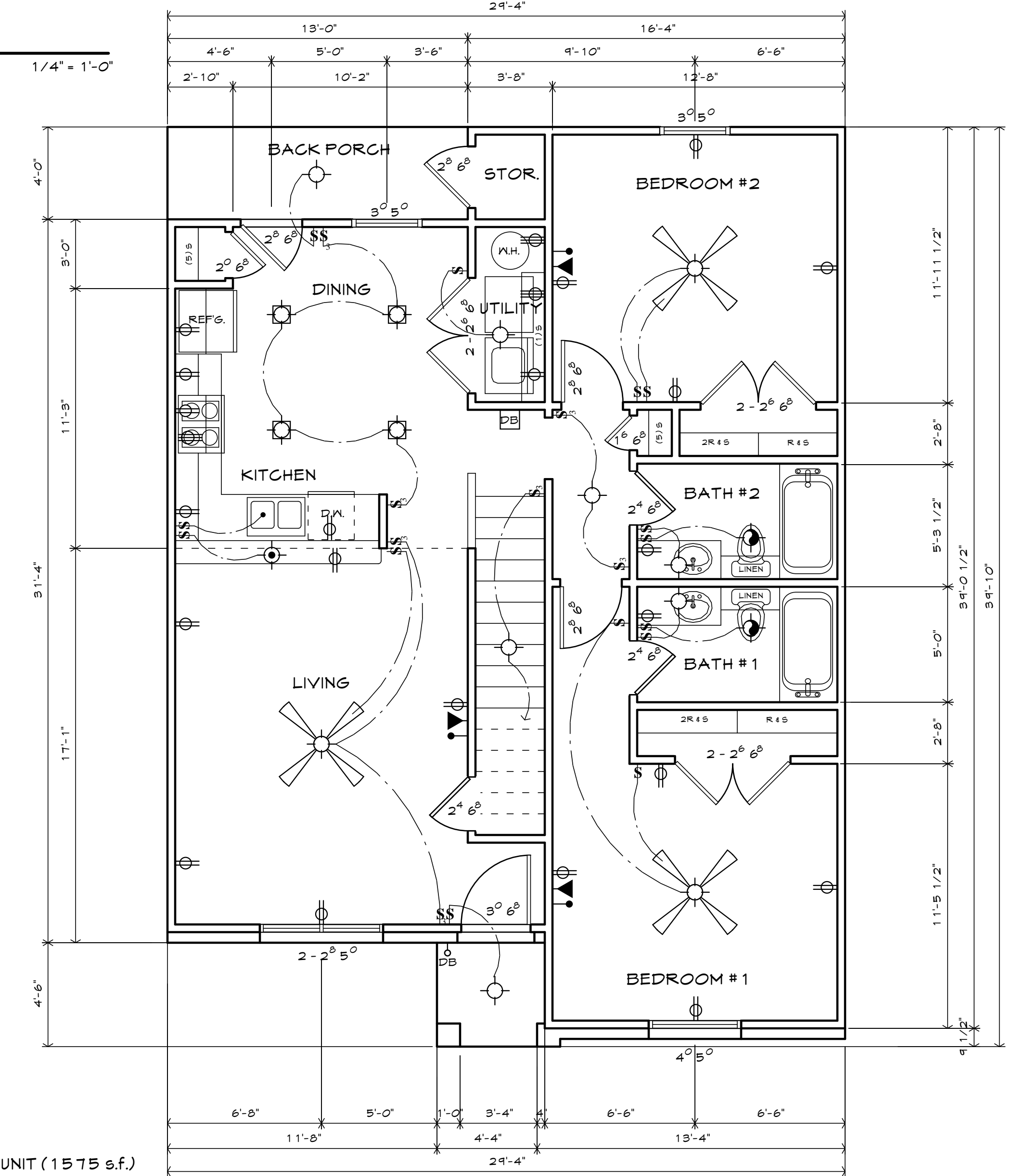
① 1st FLOOR PLAN 4-4 (1043 s.f.) 1/4" = 1'-0"
