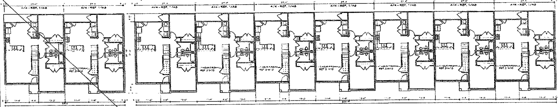
③ BLDG. C - 1st FLOOR PLAN PHASE B
