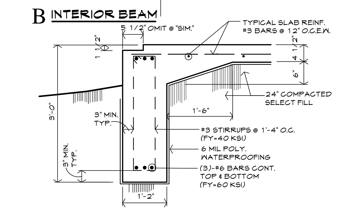
3 FOUNDATION DETAILS NOTE: GRADE BEAMS TO EXTEND MIN. 1'-0" INTO UNDISTURBED SOIL 3/4" = 1'-0"
