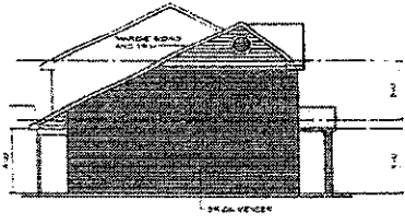
5 BLDG. E - LEFT SIDE ELEV. PHASE 1
