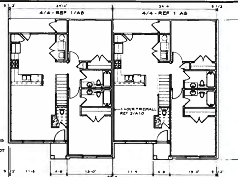
3 BLDG. C - 1st FLOOR PLAN
