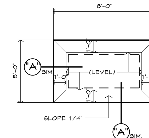
3 FOUND. PLAN MAILBOX 1/4" = 1'-0"
