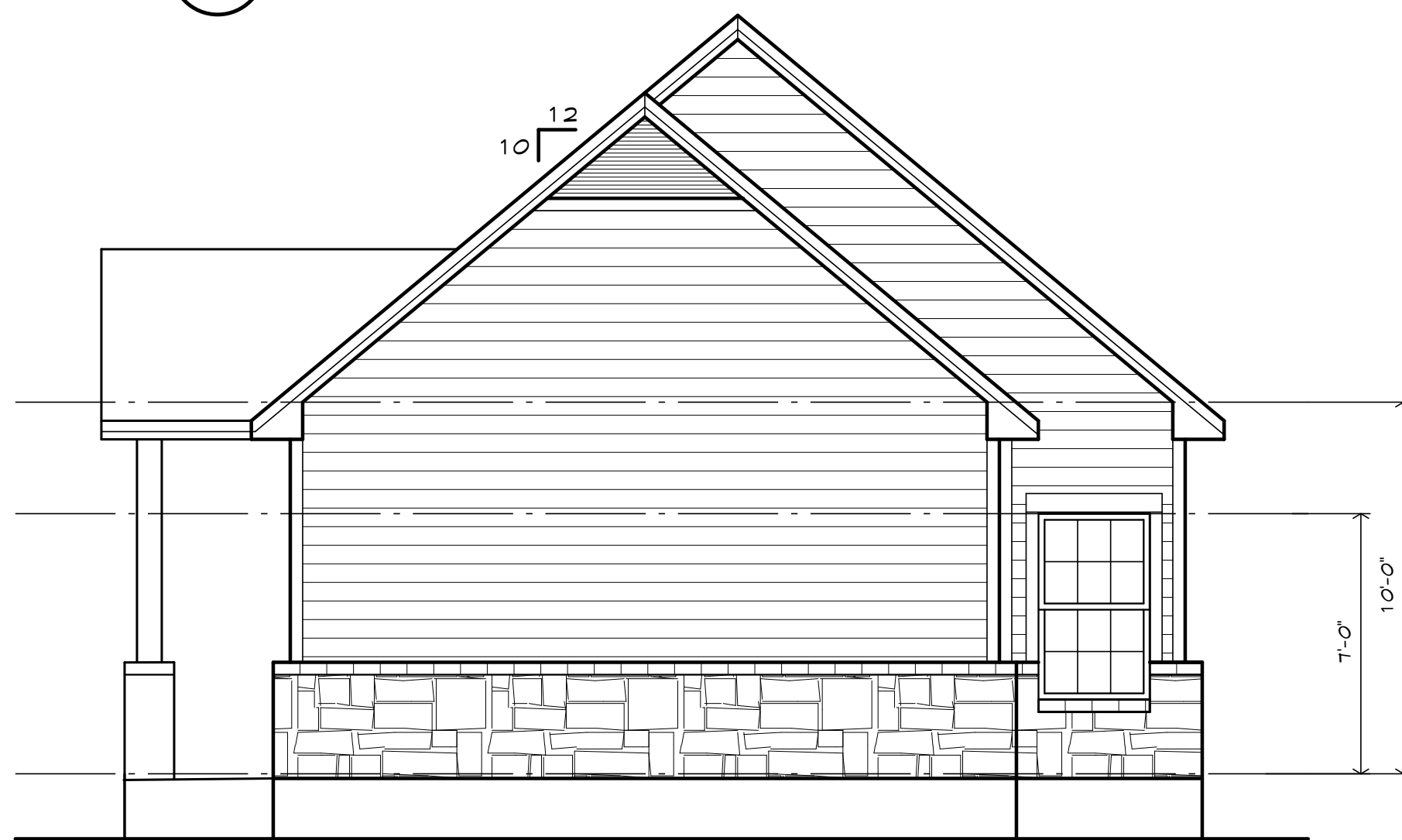
5 CLUB HOUSE SIDE ELEVATION 1/4" = 1'-0"
