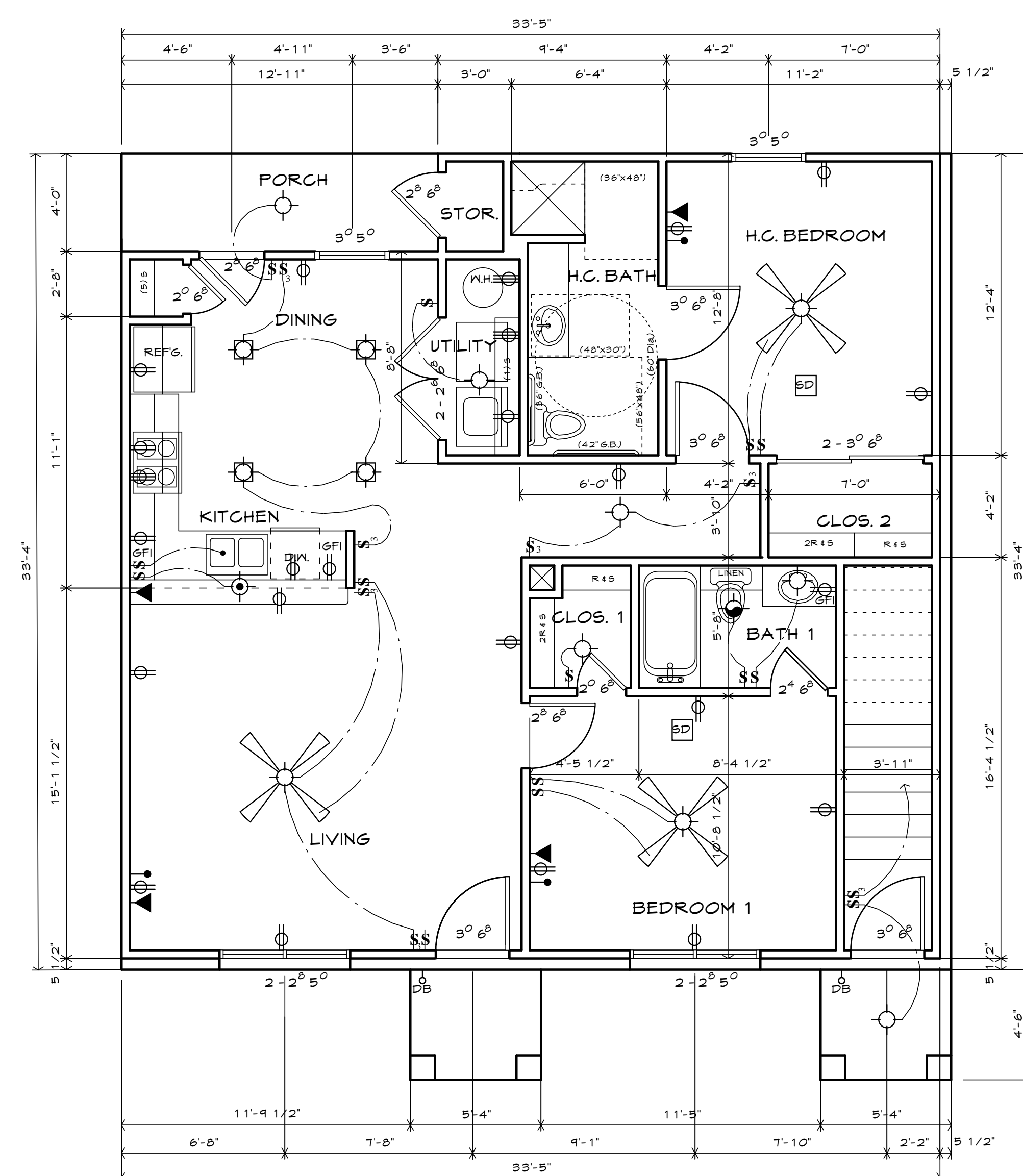
③ 1st FLOOR PLAN 2-2 "HC" Heated Area: 973 s.f. 1/4" = 1'-0"
