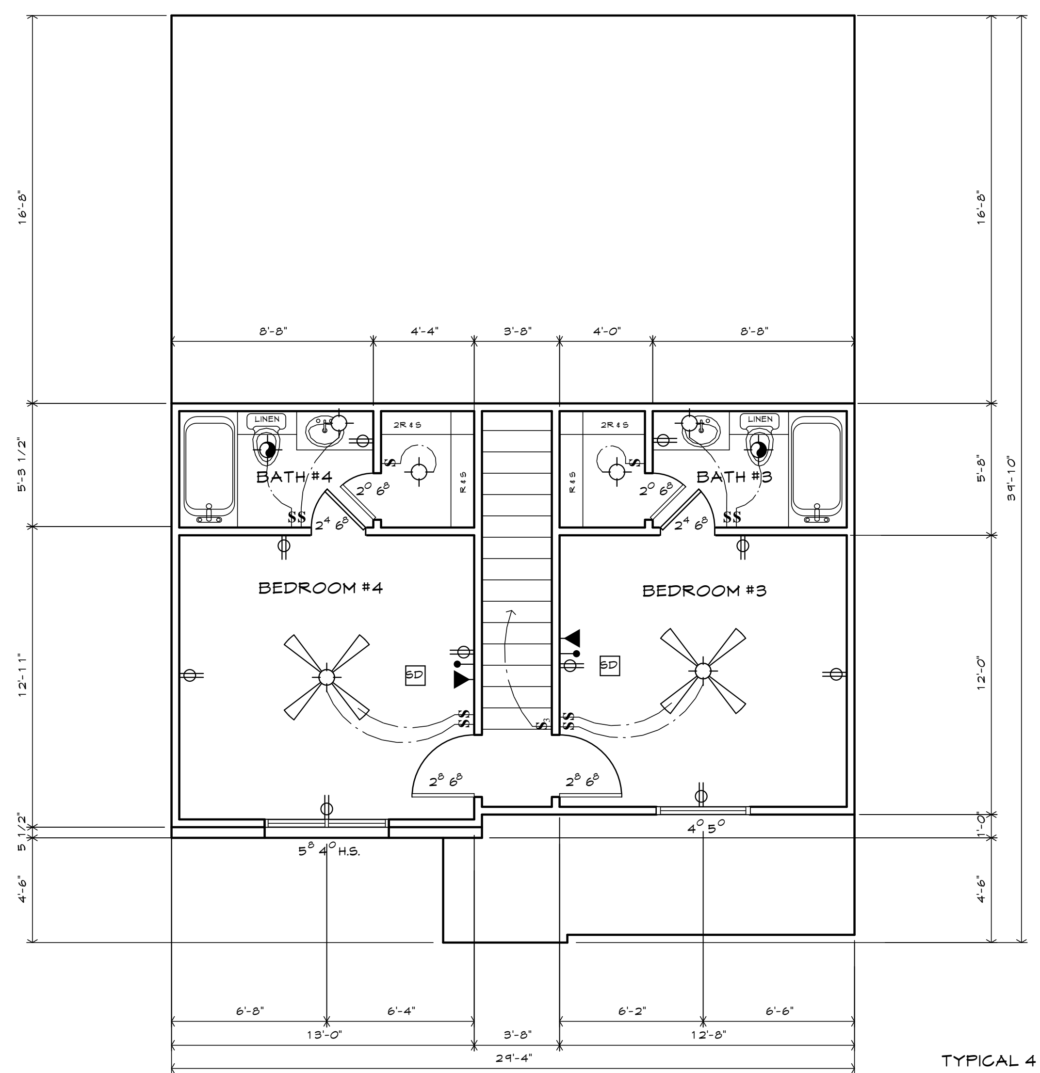
② 2nd FLOOR PLAN 4-4 (532 s.f.) 1/4" = 1'-0"
