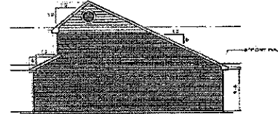
5 BLDG. A, B & C - RIGHT SIDE ELEV. 1/8" = 1'-0"
