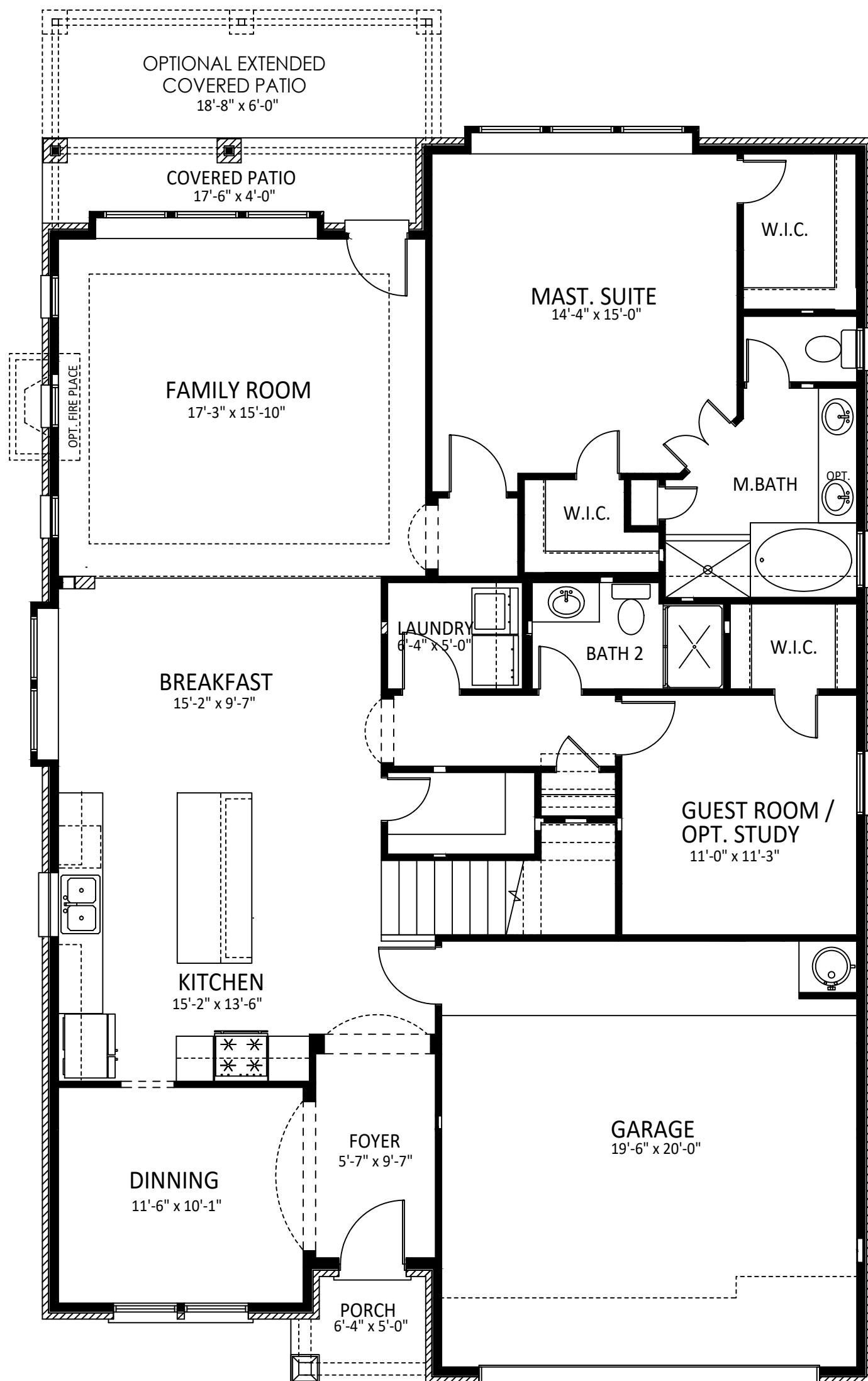
FIRST FLOOR
