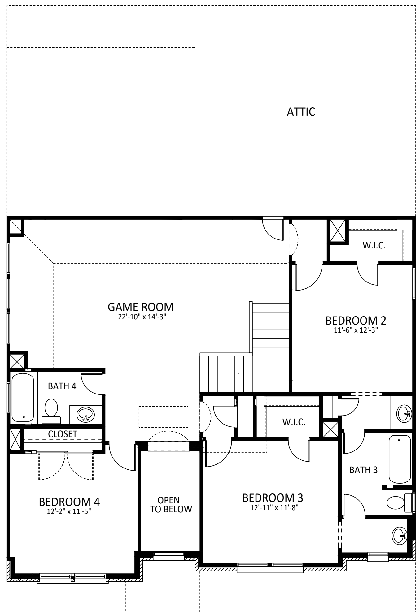
SECOND FLOOR
