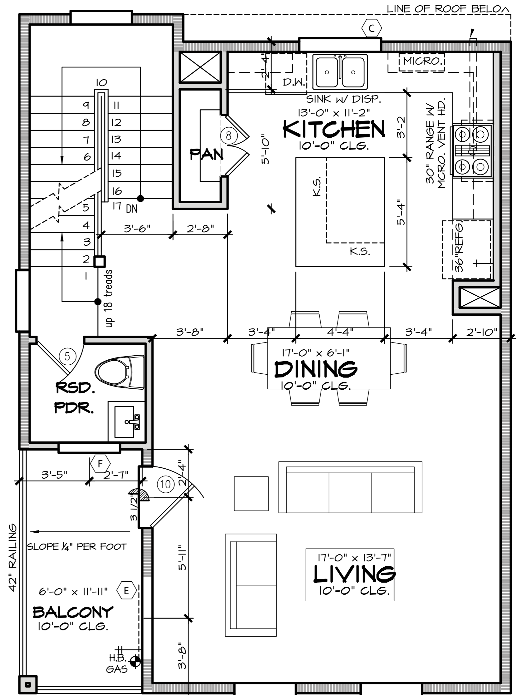
SECOND FLOOR
