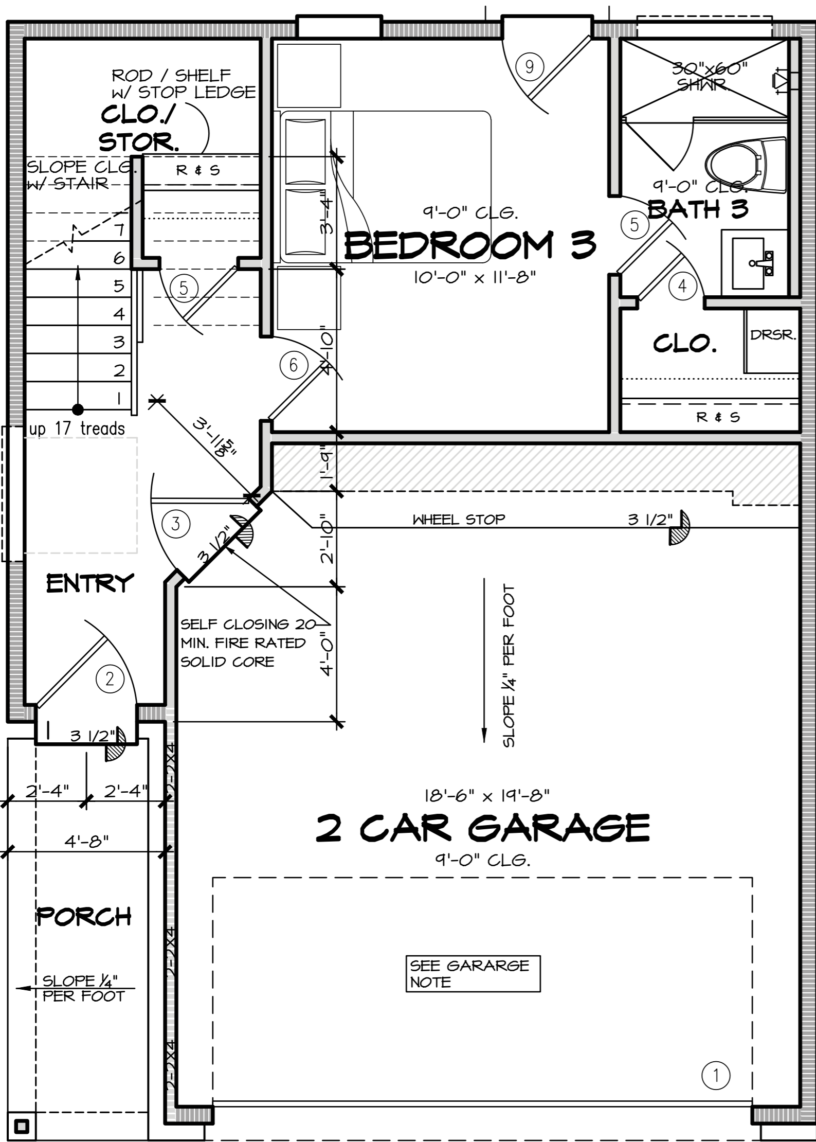
FIRST FLOOR
