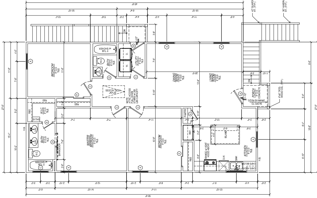
FLOOR PLAN-2ND FLOOR
