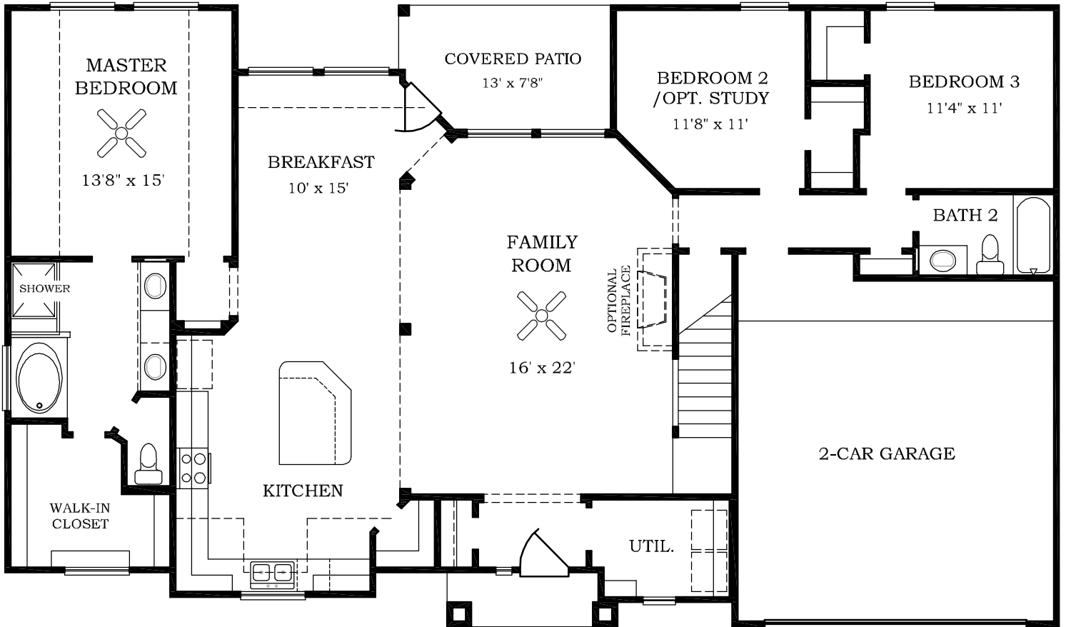
FIRST FLOOR
