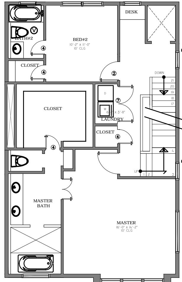
THIRD FLOOR PLAN (C)
