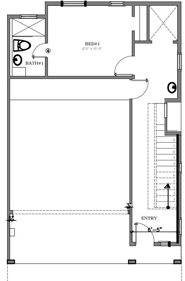
FIRST FLOOR PLAN (A)
