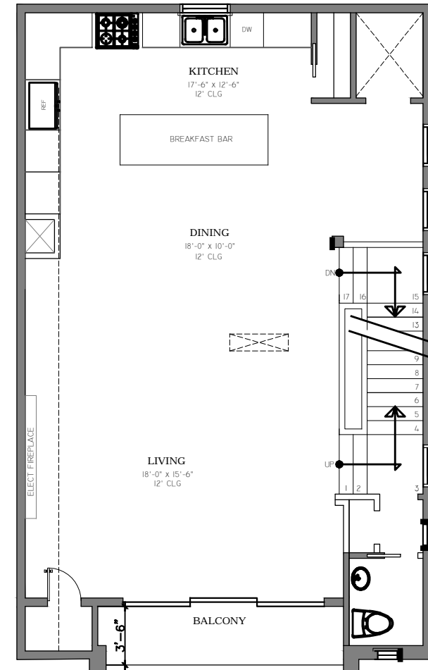
SECOND FLOOR PLAN (B)
