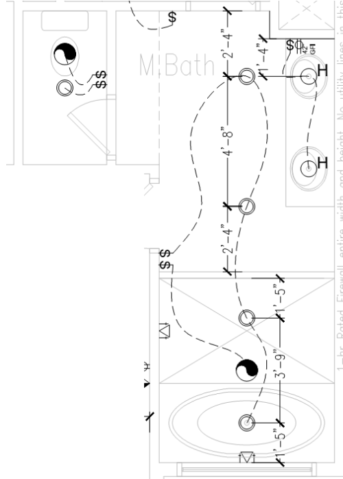
Master Bath Floor Plan
