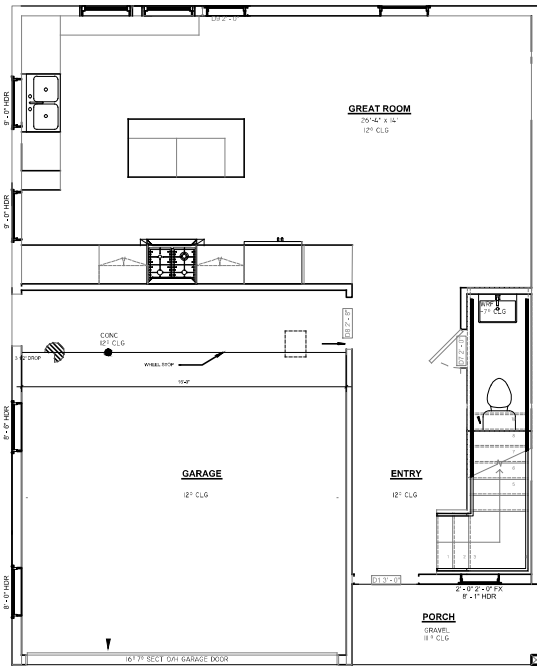
FIRST FLOOR PLAN (A) 554sf
