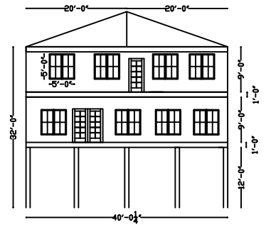
ELEVATION - PLAN NORTH PROPOSED CHANGE
