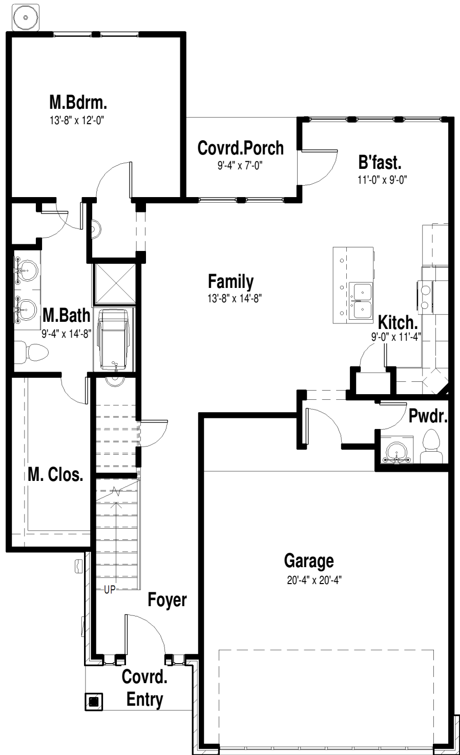
1 FIRST FLOOR PLAN-brochure
