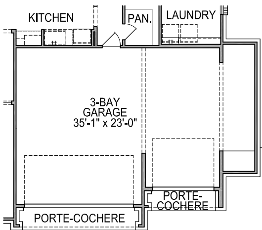
FIRST FLOOR PLAN OPT. #0613 5' GARAGE EXT.
