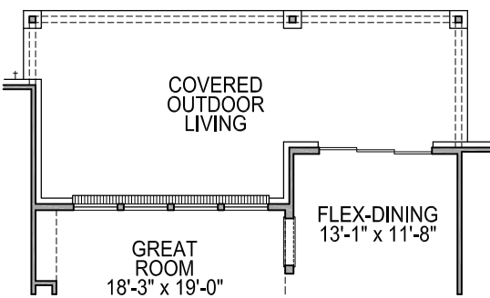
FIRST FLOOR PLAN OPT. #0789 EXT. COVERED OUTDOOR LIVING W/ SLIDERS @ FLEX-DINING
