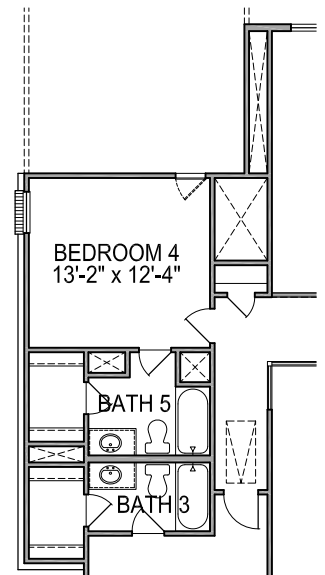
SECOND FLOOR PLAN OPT. #0567 BATH 5
