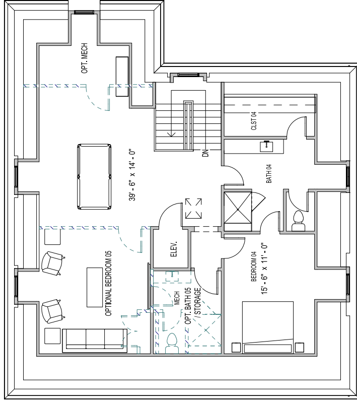
01 GRAPHIC THIRD FLOOR PLAN
