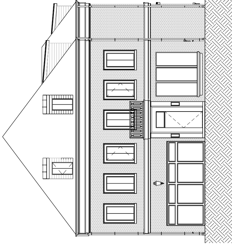
01 FRONT ELEVATION GRAPHIC SCALE: 1/8" = 1'-0"
