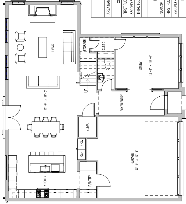
01 GRAPHIC - FIRST FLOOR PLAN
