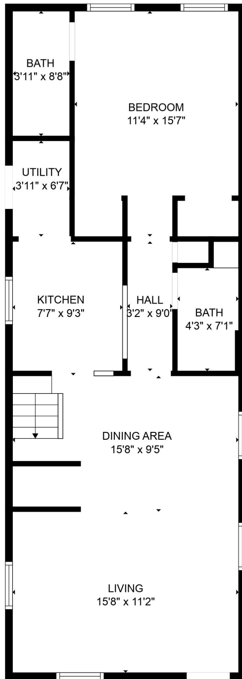
FLOOR 1
