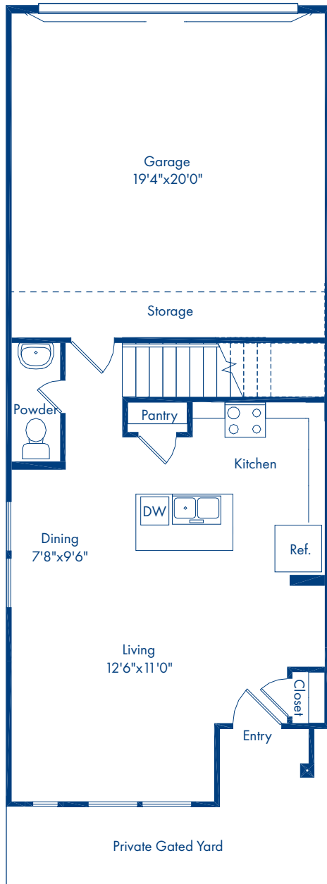
FIRST FLOOR
