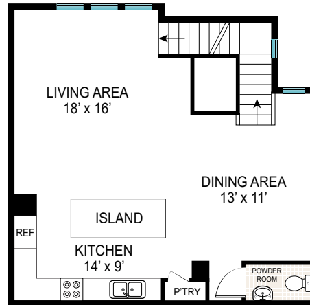
2ND FLOOR
