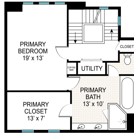
3RD FLOOR
