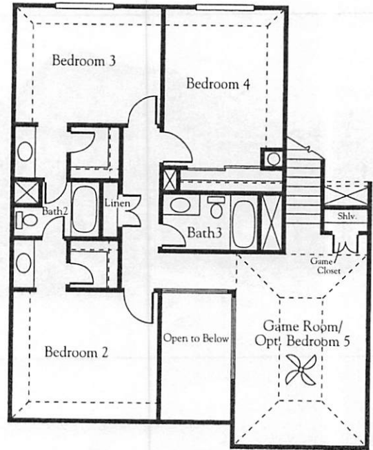
SECOND FLOOR
