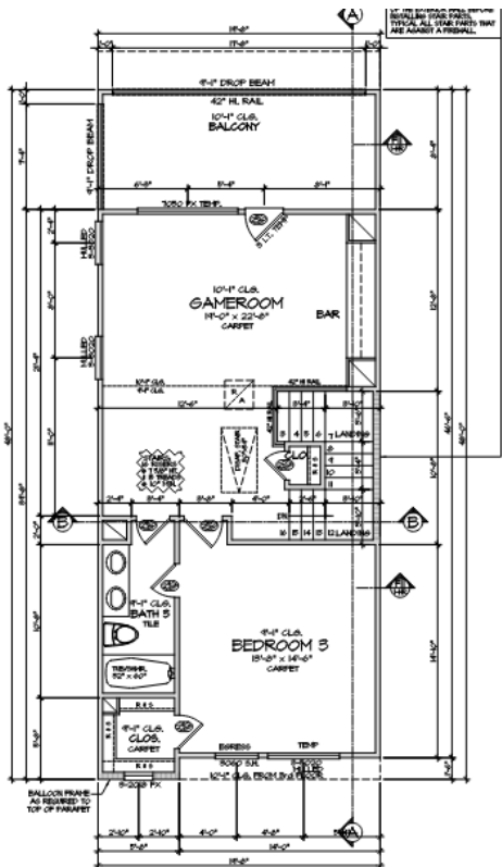
THIRD FLOOR PLAN SCALE: 1/4" = 1'-0"
