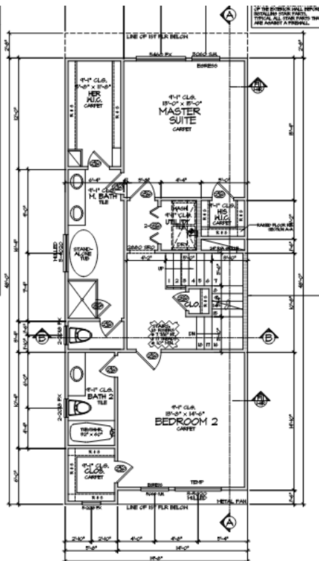
SECOND FLOOR PLAN SCALE: 1/4" = 1'-0"
