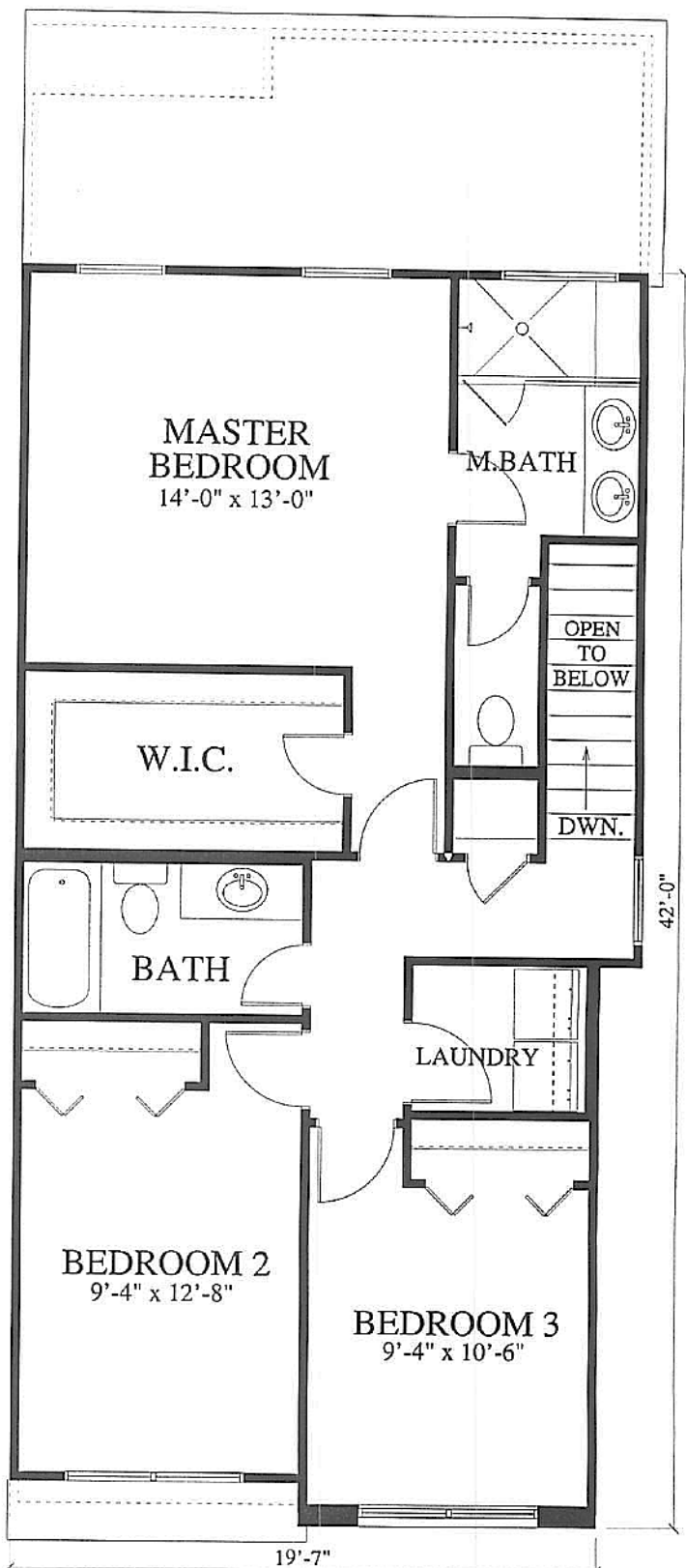
SECOND FLOOR PLAN 804 S.F.
