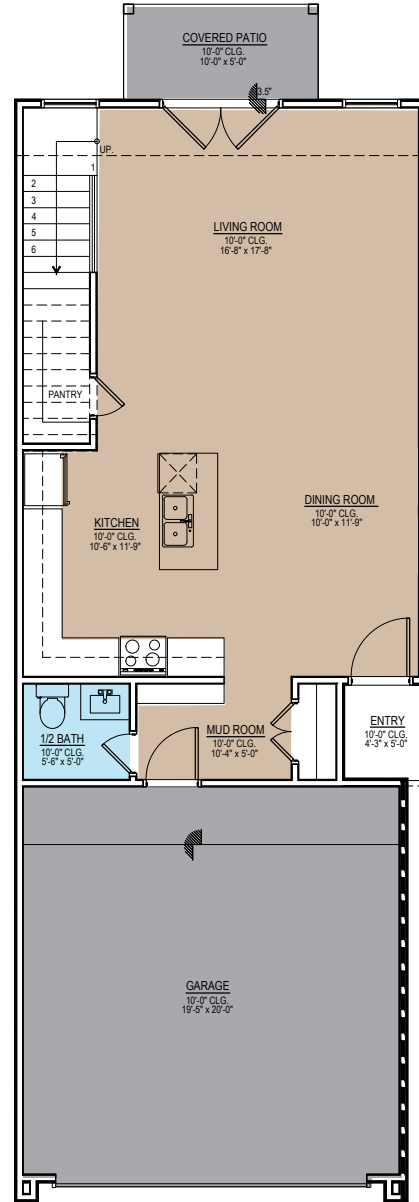
NORTH UNIT 1 1 FIRST FLOOR PLAN 1/4"=1'-0"
