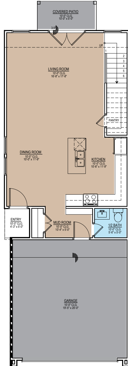
NORTH 1 UNIT 2 FIRST FLOOR PLAN 1/4"=1'-0"
