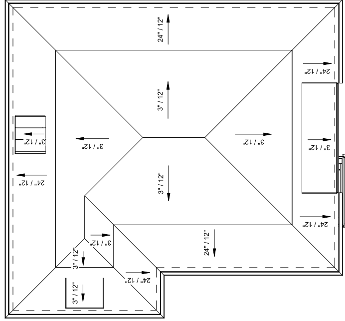
2 ROOF GRAPHIC PLAN - B1.b SCALE: 1/8" = 1'-0"
