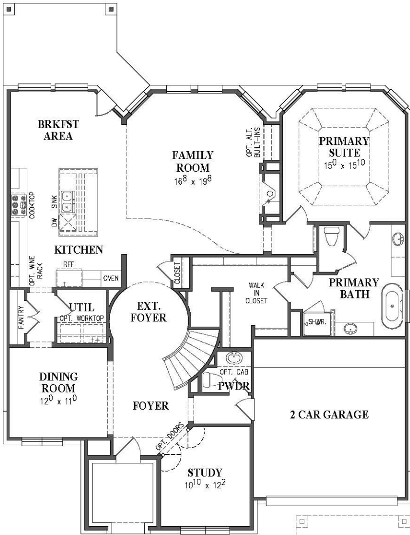
FIRST FLOOR
